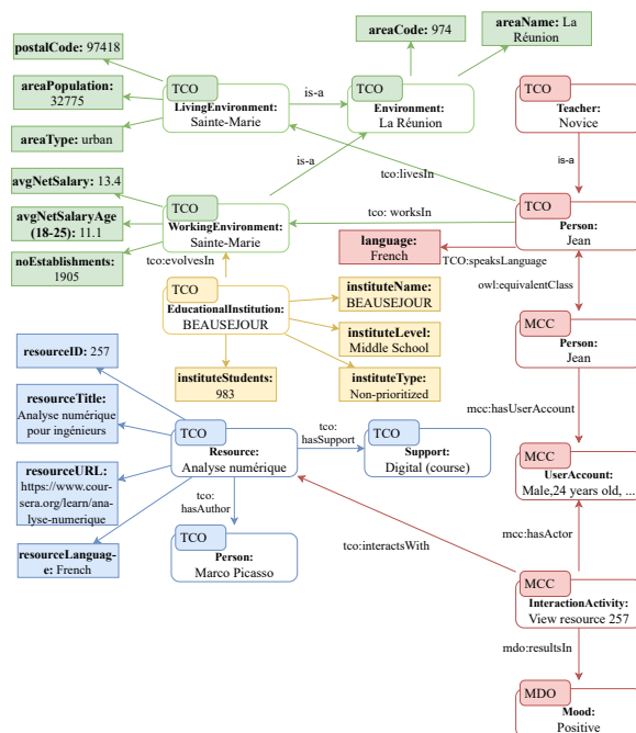
Fig. 4. An ABox ontology example
