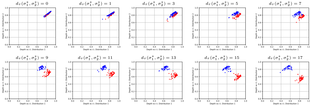
Figure 9: DD -plots for pairs of distributions stemming from different instances of the location-shift model . The two distributions contain 50 observations each, drawn from two Mallows models using Kendall \tau distance with parameter \phi_1 = \phi_2 = e^{-1} . Difference between locations is indicated in each individual plot.
