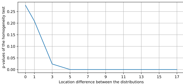
Figure 10: p -values (averaged over 100 random repetitions) for the test of homogeneity for a pair of Mallows distributions stemming from the location-shift model with location difference d_\tau(\sigma_1^*, \sigma_2^*) \in \{0, \dots, 17\} .
