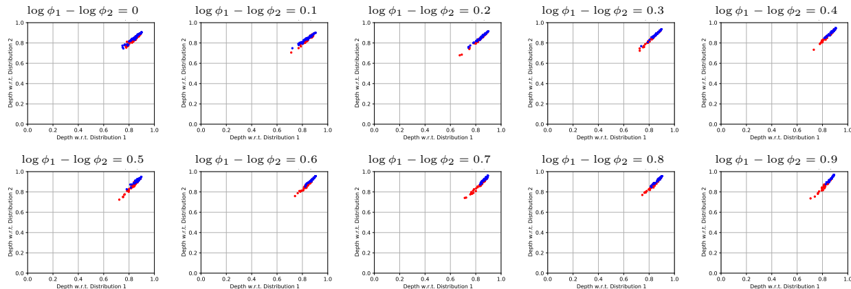
Figure 11: DD -plots for pairs of distributions stemming from different instances of the scale-difference model . The two distributions contain 50 observations each, drawn from two Mallows models (using Kendall \tau distance) with the same center and with parameters \phi_1 = e^{-1} and \phi_2 = e^\psi where \psi \in \{-1, -1.1, -1.2, -1.3, -1.4, -1.5, -1.6, -1.7, -1.8, -1.9\} . Difference between scales' logarithms is indicated in each individual plot.
