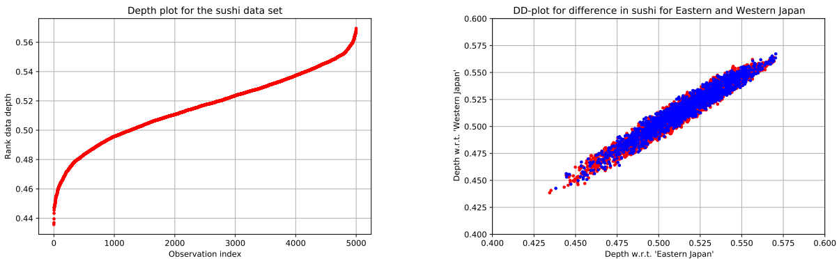
Figure 14: Exploratory statistics of the Sushi data set by [35] ( https://www.kamishima.net/sushi/ ). Left: The depth of each observation in the set, in increasing depth order. Right: The comparative DD -plot for Eastern (red) and Western (blue) Japan.
