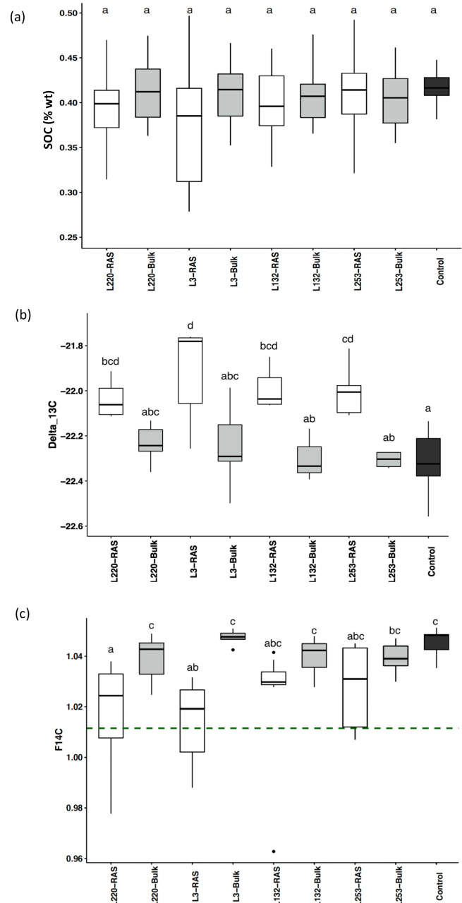
Figure 1. (a) Soil organic carbon (SOC) content of the RAS (root-adhering soil), bulk soil and unplanted control soil. (b) \delta^{13}\text{C} ‰ in the RAS, bulk soil and unplanted control soil. (c) F^{14}\text{C} in the RAS, bulk soil and unplanted control soil. The dotted line indicates the F^{14}\text{C} value of pearl millet tissue, i.e. the new carbon F^{14}\text{C} ( F^{14}\text{C} = 1.012 \pm 0.002 ). Different letters indicate significant difference using a Tukey post hoc test ( p < 0.05 ).
