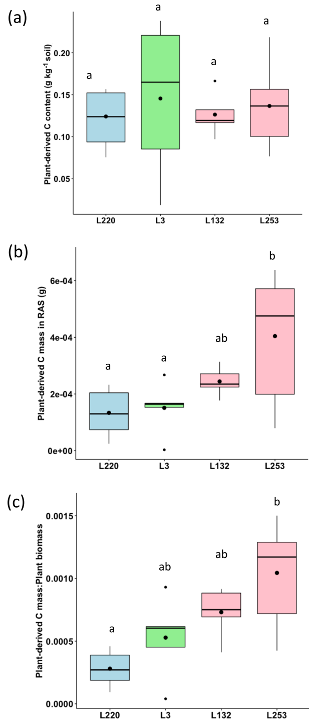
Figure 2. (a) Plant-derived carbon content (PDCC; g C kg -1 soil) in the root-adhering soil (RAS) of the four pearl millet lines. (b) Plant-derived carbon mass deposited (PDCD; g C) in the RAS of the four pearl millet lines. (c) Ratio between the plant-derived carbon mass and the total plant biomass produced by the four pearl millet lines. Black points within the boxes represent the means. Different letters indicate significant differences using an ANOVA and the Tukey post hoc test ( p < 0.05 ).
