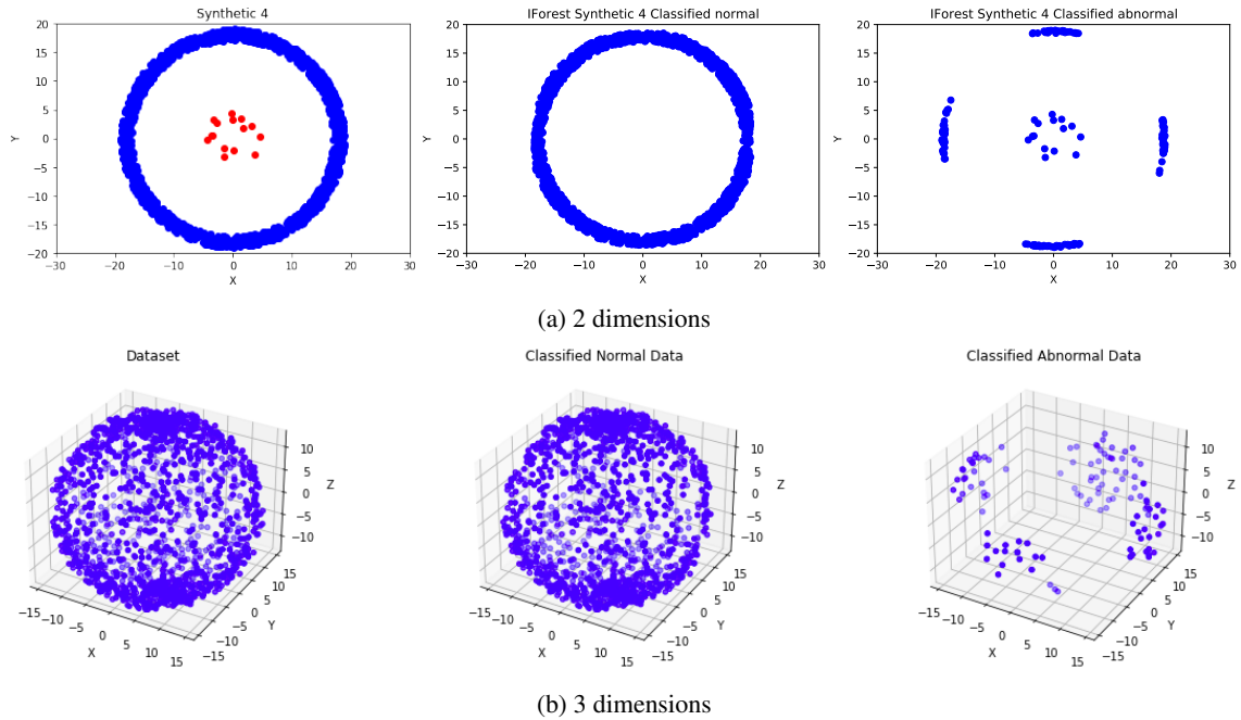
FIGURE 13: IForest results on datasets of dimensions 2 and 3.
