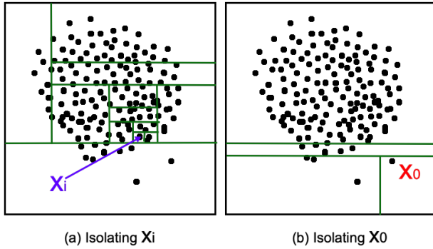
FIGURE 1: Anomalies ( X_0 ) are isolated faster than normal data ( X_i ).
