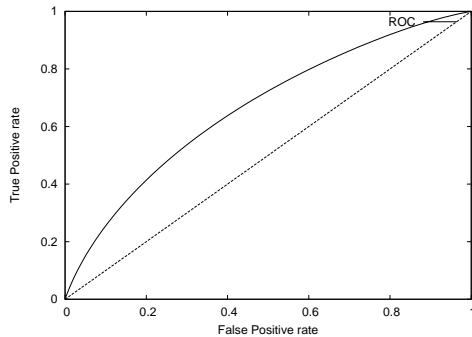
FIGURE 8: ROC Curve.
