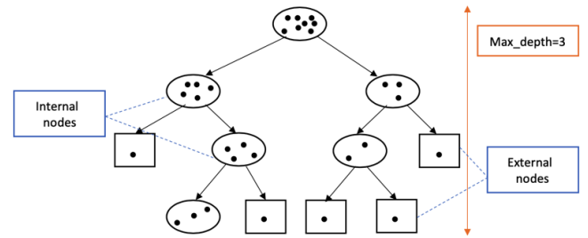
FIGURE 2: itree example, \psi = 8 .
