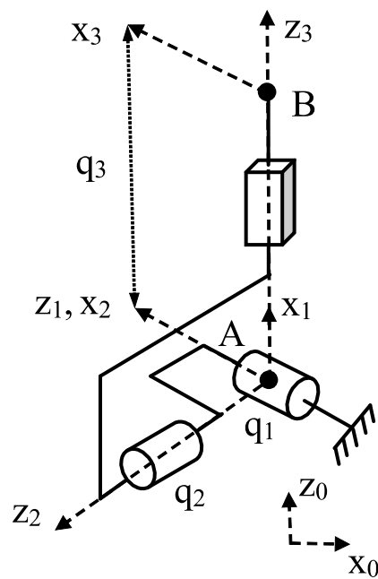
Figure 2. Example of an RRP serial robot
