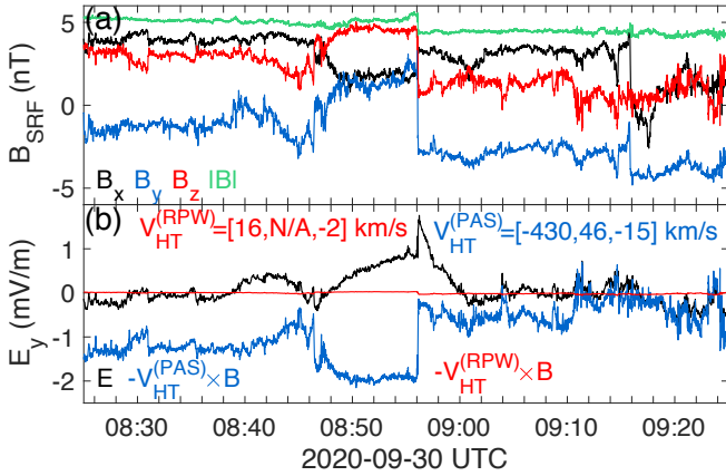
Fig. 4. Example of a failed HT analysis due to bad E_y data. Same format as Figs. 2a,b.
