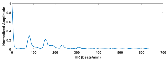
Fig. 8. The frequency spectrum computed from the predicted BVP signal by our BVPNet.
