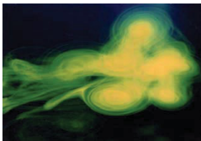
Fig. 1. Top view of the zigzag instability destructuring a vertical vortex dipole [2].
