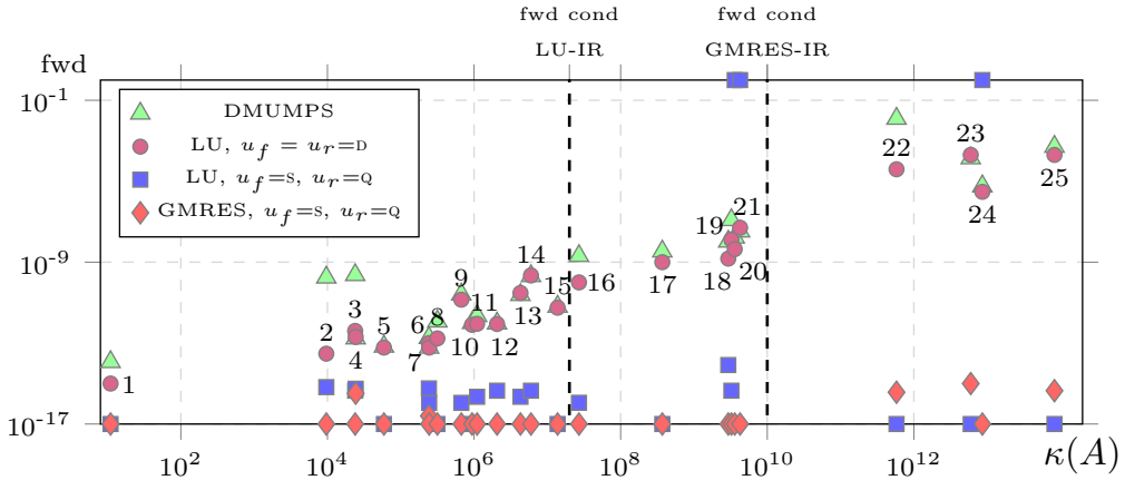
Fig. 1. Forward error achieved by three IR variants for the matrices used in Table 2 (denoted by their ID) as a function of their condition number \kappa(A) . We fix u = u_g = u_p = \text{D} . The vertical dashed lines show the forward convergence condition for LU-IR ( u_f = s, u_r = \text{D} ) and for GMRES-IR ( u_f = s, u_r = u_g = u_p = \text{D} ).
