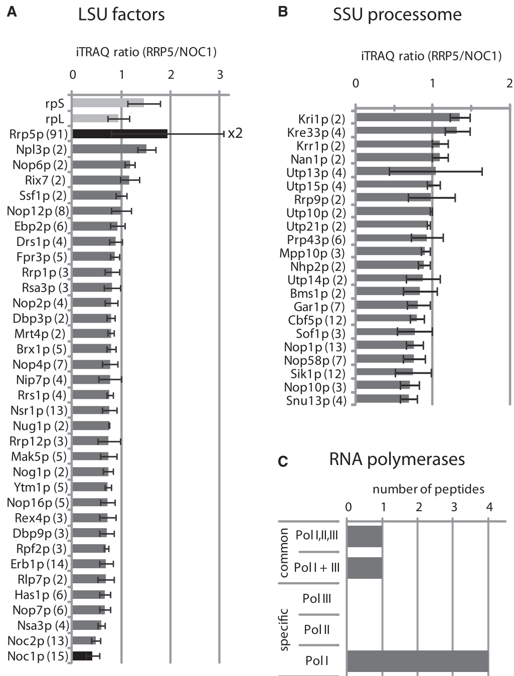
Figure 5. Comparative proteome analysis of Noc1p and Rrp5p containing pre-ribosomes. Proteins from aliquots of Noc1p-TAP and Rrp5p-TAP purifications (Figure 4) were digested using trypsin and the resulting peptides were labelled with iTRAQ(R) reagents 116 (Noc1p purification) and 117 (Rrp5p purification), subsequently pooled, separated by reversed phase nano HPLC and spotted on a MALDI-MS/MS target. The top eight peptides of the MS run in each spot were selected for fragmentation in MS/MS mode to determine the sequence of the peptide and the ratio of the iTRAQ reporter group signal intensities (117/116). For proteins identified with more than one peptide [ion score confidence interval (CI) >95%] the average iTRAQ ratio (117/116 = RRP5/NOC1) was calculated. LSU biogenesis factors (A) and SSU processome components (B) identified in both purifications are listed according to their average iTRAQ ratio (error bars are standard deviations of the average ratio; numbers of identified peptides are indicated in brackets). The average iTRAQ ratios of ribosomal proteins of the large (rpL) and the small (rpS) subunit identified with more than one peptide are shown in (A). (C) Peptide count analysis of RNA polymerase subunits identified in both purifications. Only peptides of Pol-I-specific subunits (A12.2, A49, A135, A190) and of common subunits (AC40, ABC23) were identified with a score >95% CI (one peptide each).
