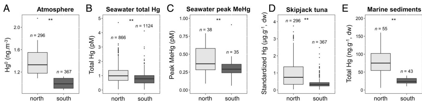
Fig. 3. Hemispheric mercury gradients in different Pacific Ocean reservoirs. The boxplots illustrate the hemispheric gradient of (A) atmospheric \text{Hg}^0 model estimates ( \text{nanograms}\cdot\text{meters}^{-3} ) extracted at tuna sampling locations (see Materials and Methods ), (B) observed total Hg concentrations ( \text{picomolar} ) in seawater (12, 34, 38, 53, 54, 56), (C) observed MeHg concentrations at peak ( \text{picomolar} ) in seawater (12, 34, 53–57), (D) standardized total Hg concentrations ( \text{micrograms}\cdot\text{grams}^{-1} , dw) in skipjack tuna (this study), and (E) observed total Hg concentrations ( \text{nanograms}\cdot\text{grams}^{-1} , dw) in marine sediments (2, 73–78). ** indicates significant differences between the northern and southern hemispheres (Kruskal–Wallis test; P < 0.01 ).
