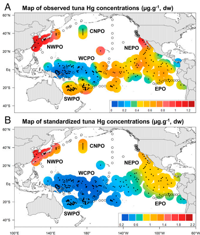
Fig. 2. Spatial variability of skipjack mercury concentrations. Smoothed spatial contour maps of (A) observed and (B) standardized Hg concentrations ( \mu\text{g}\cdot\text{g}^{-1} , dw) in skipjack white muscle samples from the Pacific Ocean. The black dots represent the location of skipjack samples. Ocean areas correspond to the sample origin: NWPO, CNPO, NEPO, EPO, SWPO, and WCPO. The transparent dots represent the location of seawater samples with available and published MeHg data (see Materials and Methods ).
