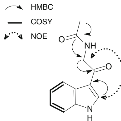
Fig. 2 HMBC, COSY and NOE correlations of compound 1
