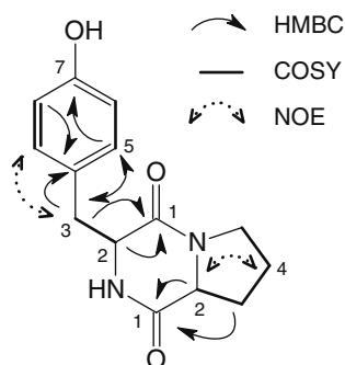
Fig. 5 HMBC, COSY and NOE correlations of compound 4
