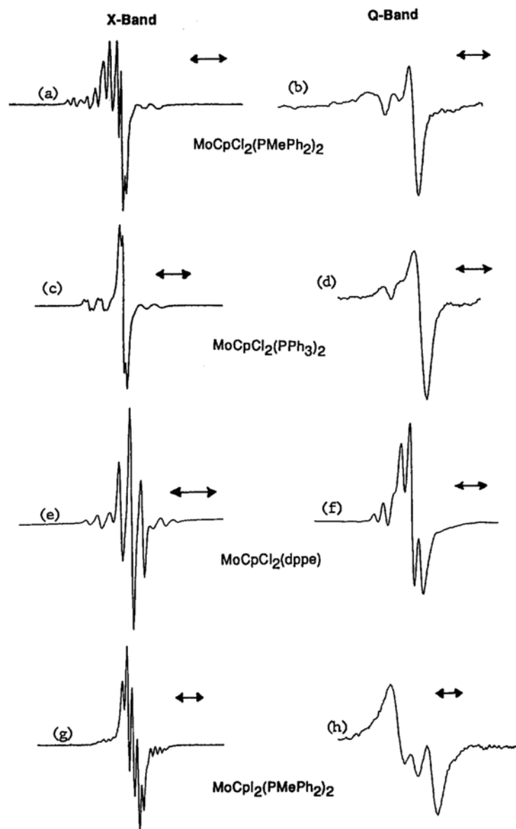
Fig. 1. Room-temperature EPR spectra of \text{CpMoX}_2\text{L}_2 complexes in \text{CH}_2\text{Cl}_2 : (a) and (b) \text{X} = \text{Cl} , \text{L} = \text{PMePh}_2 ; (c) and (d) \text{X} = \text{Cl} , \text{L} = \text{PPh}_3 ; (e) and (f) \text{X} = \text{Cl} , \text{L}_2 = \text{dppe} ; (g) and (h) \text{X} = \text{I} , \text{L} = \text{PMePh}_2 . (a), (c), (e) and (g) are X-band spectra; (b), (d), (f) and (h) are Q-band spectra. Spectra are not shown on the same g scale. Refer to Table 1 for g values and hyperfine splitting parameters.
