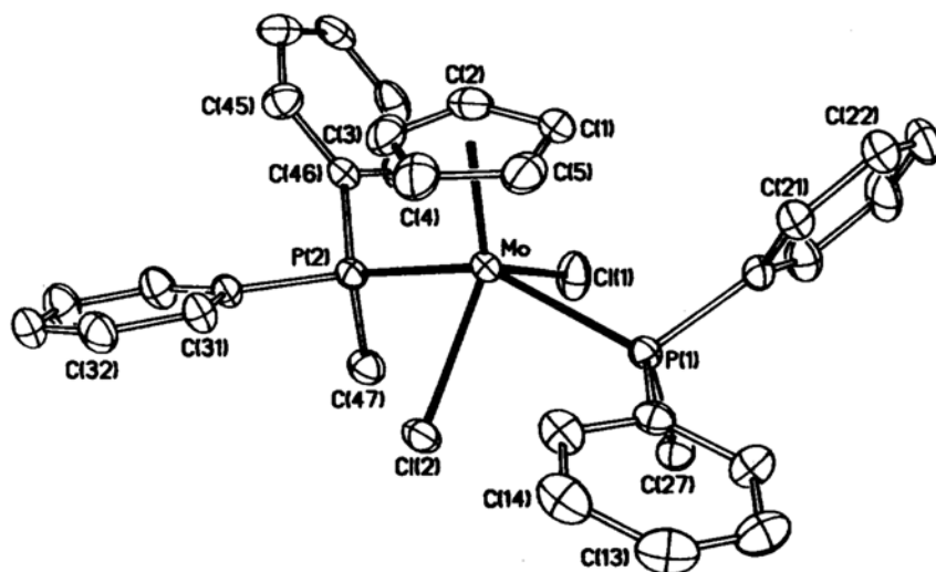
Fig. 2. An ORTEP view of the \text{CpMoCl}_2(\text{PMePh}_2)_2 molecule showing the atomic numbering scheme employed. Ellipsoids are drawn at the 40% level.
