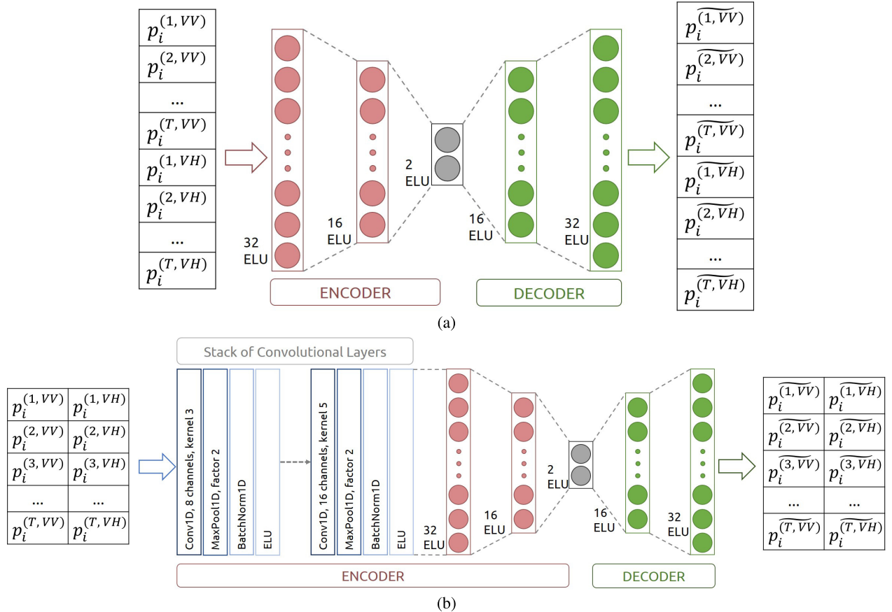
Fig. 13. Presentation of the stacked (a) AE and (b) CAE architectures for the task of modeling S1 \sigma_0 time series over Sector BXII.
