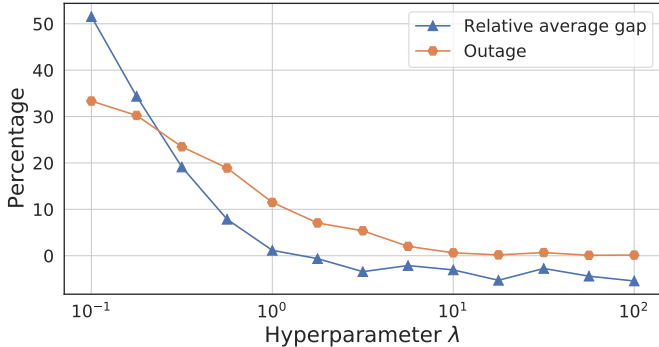
Fig. 5. Relative average gap G and outage as functions of the hyperparameter \lambda over the test set.
