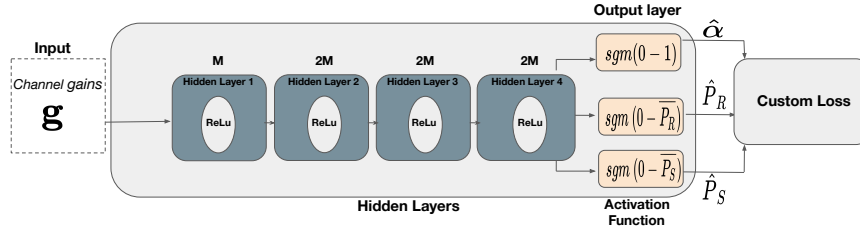
Fig. 2. Our proposed DNN architecture.
