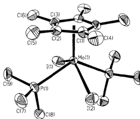
Fig. 2. Molecular view and labelling scheme for [\text{Cp}^*\text{MoCl}_{0.5}\text{I}_{1.5}(\text{PMe}_3)_2]^+ . Ellipsoids are at the 35% probability. Hydrogen atoms are not drawn.
