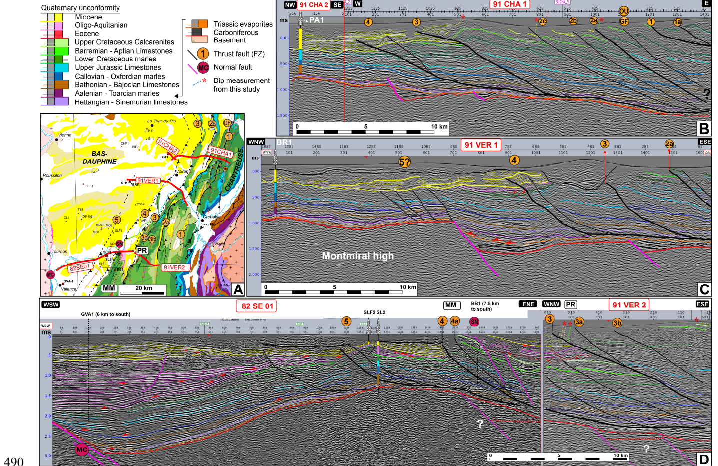
Figure 9: Seismic profiles along the Vercors and Chartreuse massifs (seismic lines published by Deville (2021) and reinterpreted). (A) Geographical and geological locations of the interpreted seismic lines. (B) Seismic profiles 91CHA1 and 91CHA2. Interpretation is proposed using PA-1 well data and fieldwork data. Note that the Outherans blind thrust [OU] corresponds further north to the
