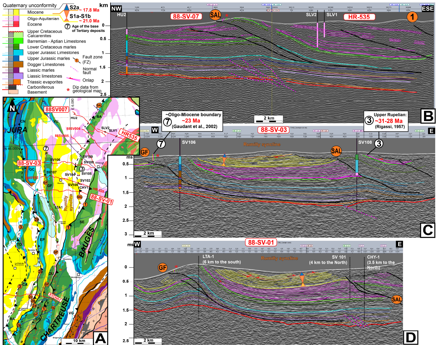
Figure 10: The salève (SAL) and Gros Foug (GF) faults between the Chartreuse massifs and the Jura synclines (A, legend in Fig. 1) as based on seismic profiles 88SV07+HR-535 (B), 88SV03 (C) and 88SV01 (D).
