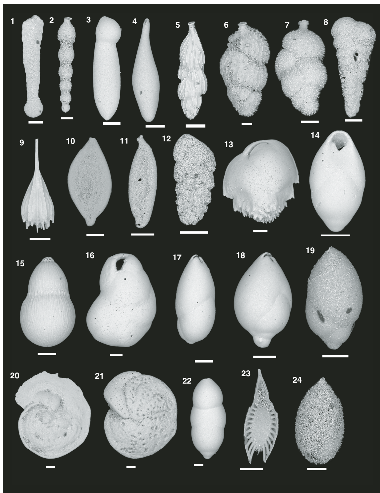
Figure F26. Benthic foraminifera, Hole U1541B. Scale bars = 100 \mu\text{m} . 1. Spiroplectella sp. (11H-CC). 2. Stilostomella lepidula . (14H-CC). 3. Pleurostomella incrassata (9H-CC). 4. Procerolagena clavata (13H-CC). 5. Uvigerina sp. (9H-CC). 6. Uvigerina peregrina (10H-CC). 7. Uvigerina hispida (13H-CC). 8. Siphotextularia sp. (13H-CC). 9. Lagena plumigera (10H-CC). 10, 11. Spiroloculina sp. (14H-CC). 12. Bolivina decussata (10H-CC). 13. Ehrenbergina sp. (11H-CC). 14. Pleurostomella sp. (14H-CC). 15. Pseudonodosaria sp. (9H-CC). 16. Evolvocassidulina sp. (6H-CC). 17–19. Globobulimina sp. (17, 18) 13H-CC. (19) 15H-CC. 20. Laticarina pauperata (14H-CC). 21. Cibicides wuellerstorfi (15H-CC). 22. Pseudoglandulina sp. (13H-CC). 23. Lagena quadralata (14H-CC). 24. Fissurina sp. (covered with nannofossils) (15H-CC).
