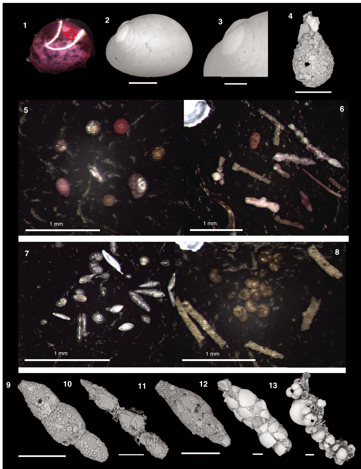
Figure F27. Agglutinated and calcareous benthic foraminifers and bivalves from mudline samples, Site U1541. Scale bars = 100 \mu\text{m} unless otherwise noted. 1. Stained bivalve (both valves intact). 2. Bivalve with concentric growth lines. 3. Bivalve beak. 4. Lagenammia sp. 5. Stained calcareous foraminifers. 6. Stained agglutinated foraminifers. 7. Unstained calcareous foraminifers. 8. Unstained agglutinated foraminifers. 9, 10. Reophax sp. 11. Astrorhiza sp. 12, 13. Rhabdammina sp.
