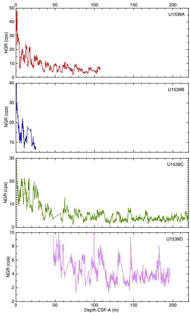
Figure F43. Natural gamma radiation (NGR) total counts, Holes U1539A–U1539D. Scales on NGR counts (y-axis) decrease from upper to lower panels.
