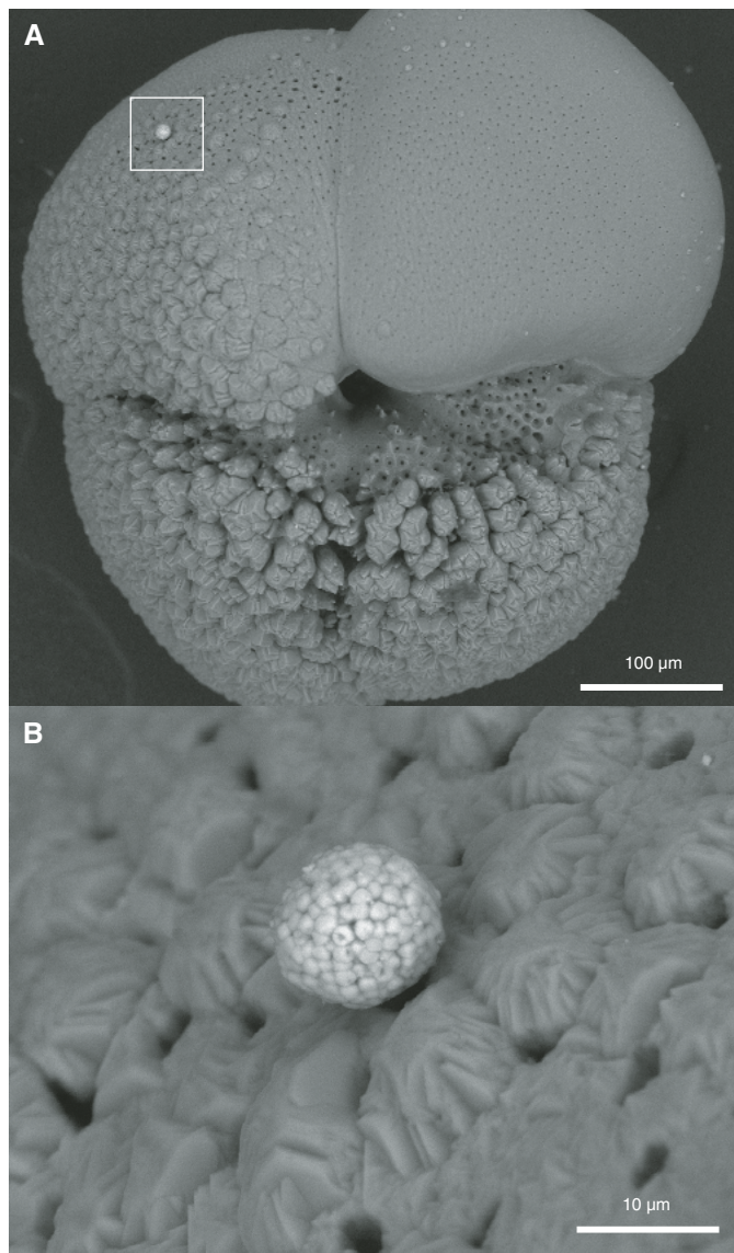
Figure F26. A. Pyrite framboid (upper left) on planktonic foraminifer Truncotalia crassaformis . B. Close-up of pyrite framboid in A.
