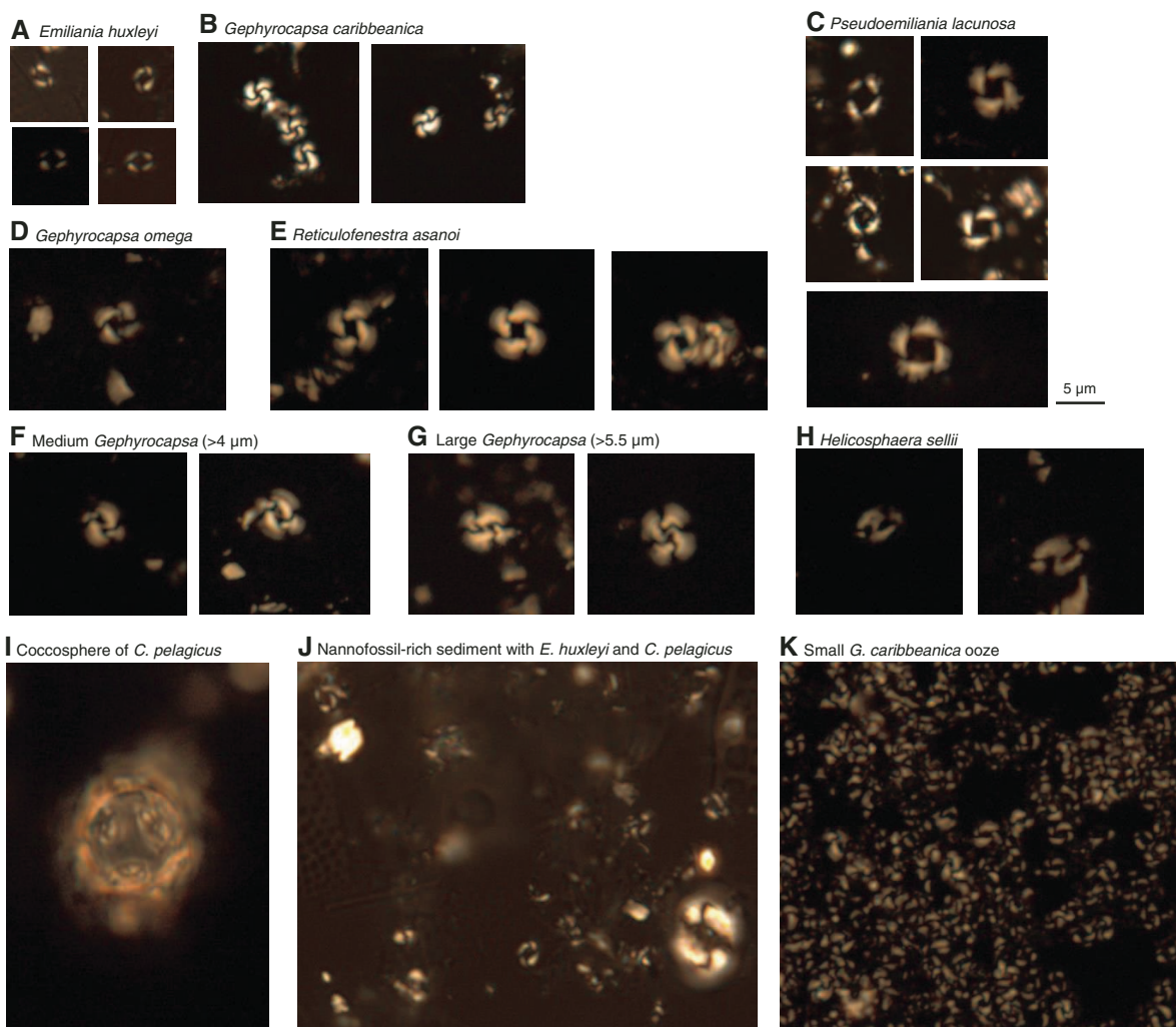
Figure F23. Calcareous nannofossils, Holes U1539A and U1539C. A. Emiliana huxleyi (383-U1539A-2H-CC). B. Gephyrocapsa caribbeanica . C. Pseudoemiliana lacunosa . D. Gephyrocapsa omega . E. Reticulofenestra asanoi . F, G. Gephyrocapsa , (F) medium (4–5.5 \mu\text{m} ), (G) large (>5.5 \mu\text{m} ). H. Helicosphaera sellii . I. Coccosphere of Coccolithus pelagicus (383-U1539C-22H-6). J. Nannofossil-rich sediment with E. huxleyi and C. pelagicus (383-U1539A-3H-CC). K. Ooze of small (<4 \mu\text{m} ) G. caribbeanica (383-U1539A-9H-CC).
