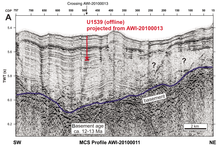
Figure F2. (A) Multichannel seismic (MCS) and (B) Parasound profiles across Site U1539.
