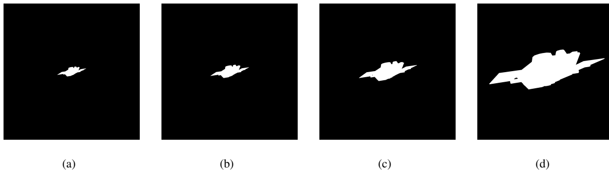
Fig. 4. Silhouette of the target satellite at 40 m (Fig.4(a)), 30 m (Fig.4(b)), 20 m (Fig.4(c)), 10 m (Fig.4(d)), for a 1024 \times 1024 pixel camera with FOV of 30^\circ . The attitude of the S/C is \varphi = 70.41^\circ , \vartheta = 66.92^\circ , \psi = -29.58^\circ
