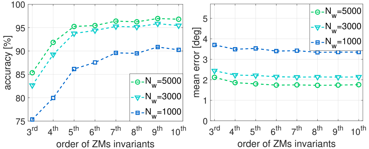
Fig. 7. Performance of the ZM invariants for different database sizes N_w .
