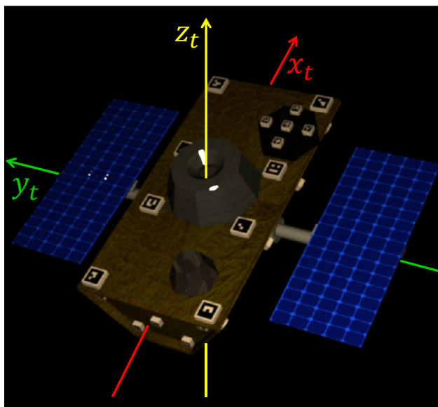
Fig. 3. Geometry and body reference frame of the target spacecraft.
