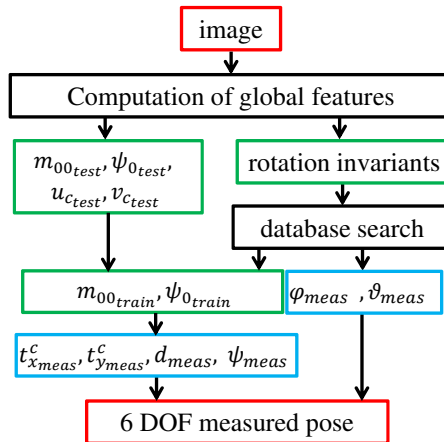
Fig. 2. Structure of the proposed pose estimation algorithm.
