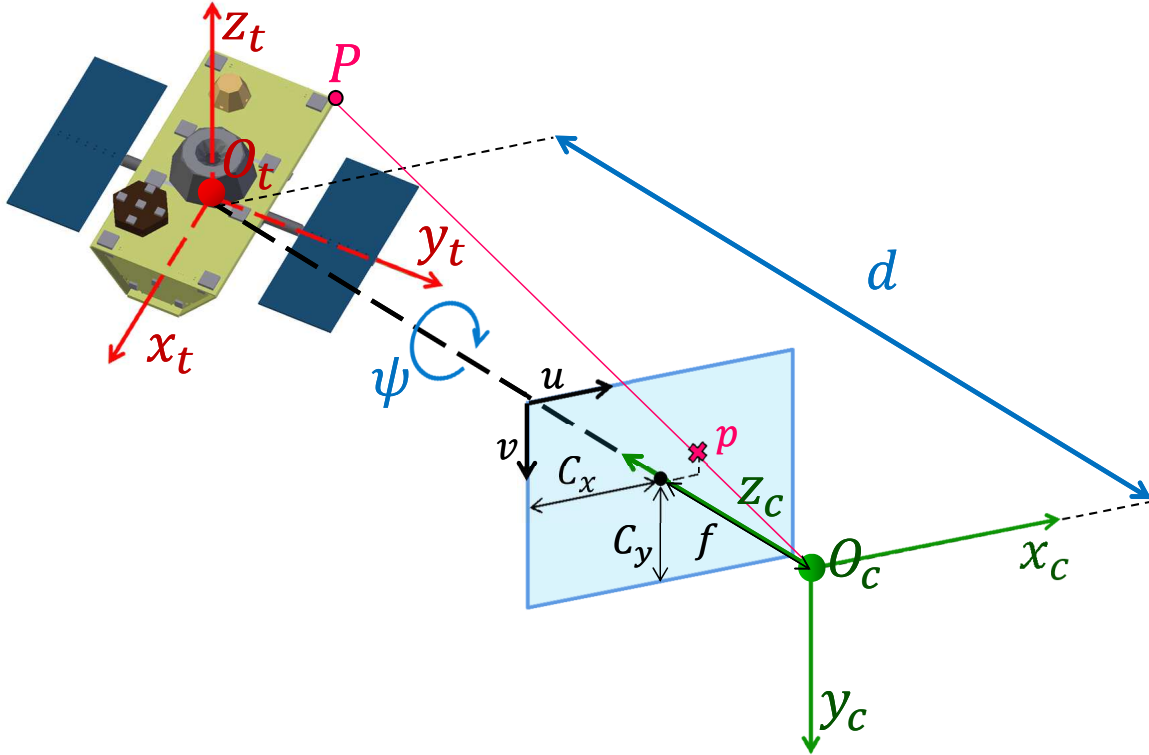
Fig. 1. Schematic representation of the pose estimation problem using a monocular image
