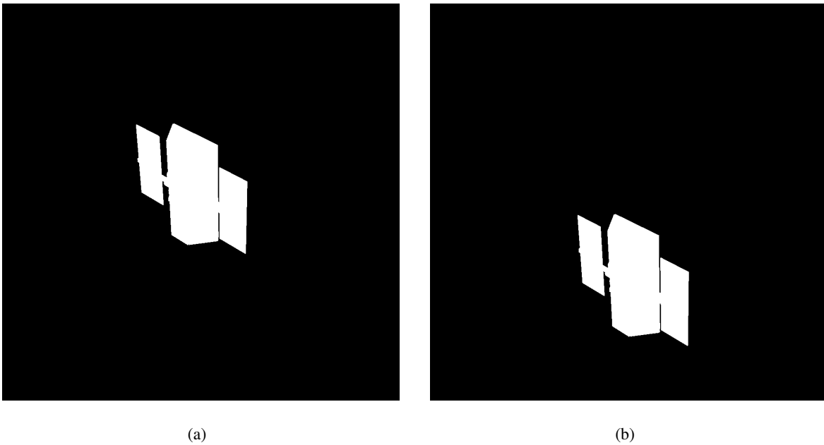
Fig. 8. Silhouette of the target satellite at 20 m, at a relative attitude of \vartheta = -35.02^\circ , \psi = 87.99^\circ . In Fig.8(a) the pointing error is \Delta\gamma = 1.43^\circ , in Fig.8(b) it is \Delta\gamma = 5.85^\circ .
