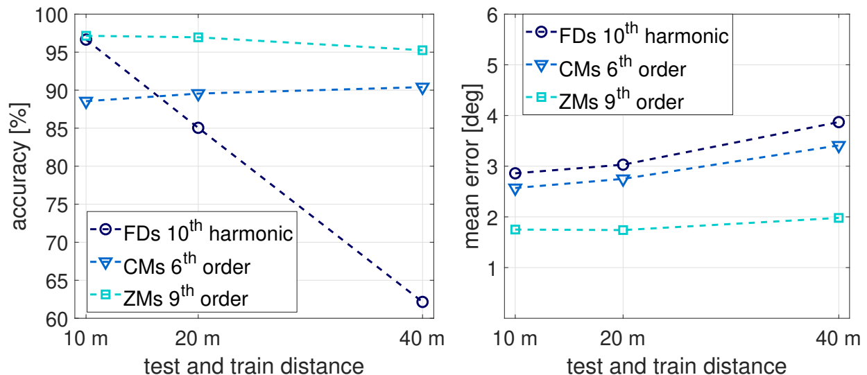
Fig. 6. Effect of a variation in the resolution of both the test and the training images ( d_{test} = d_{train} ).
