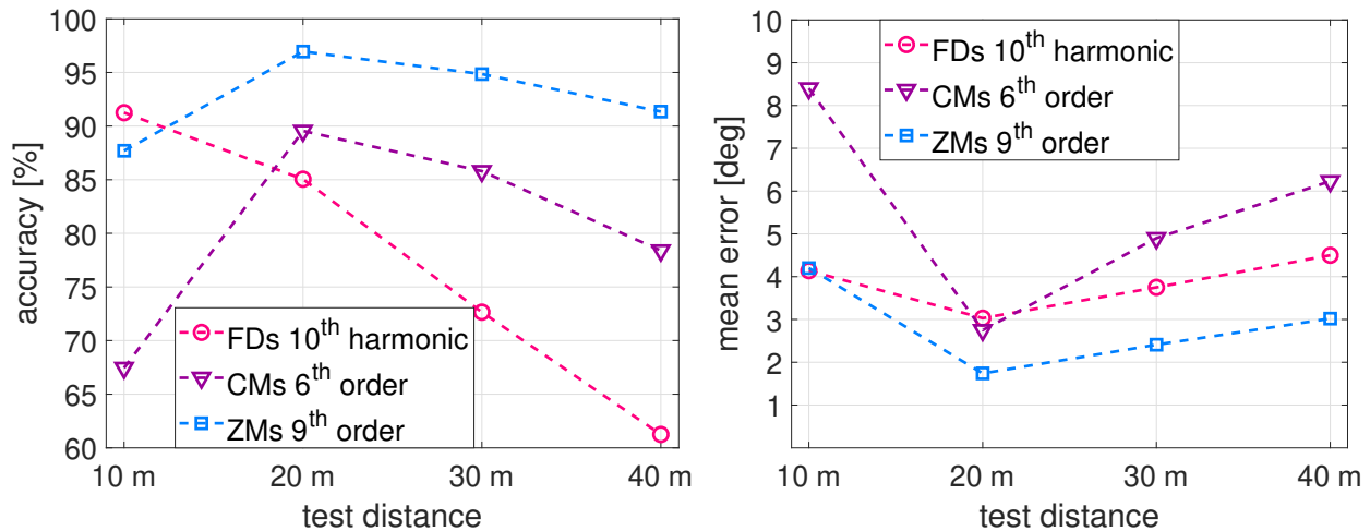
Fig. 5. Effect of a variation of the test distance with a constant training distance d_{train} = 20 m.
