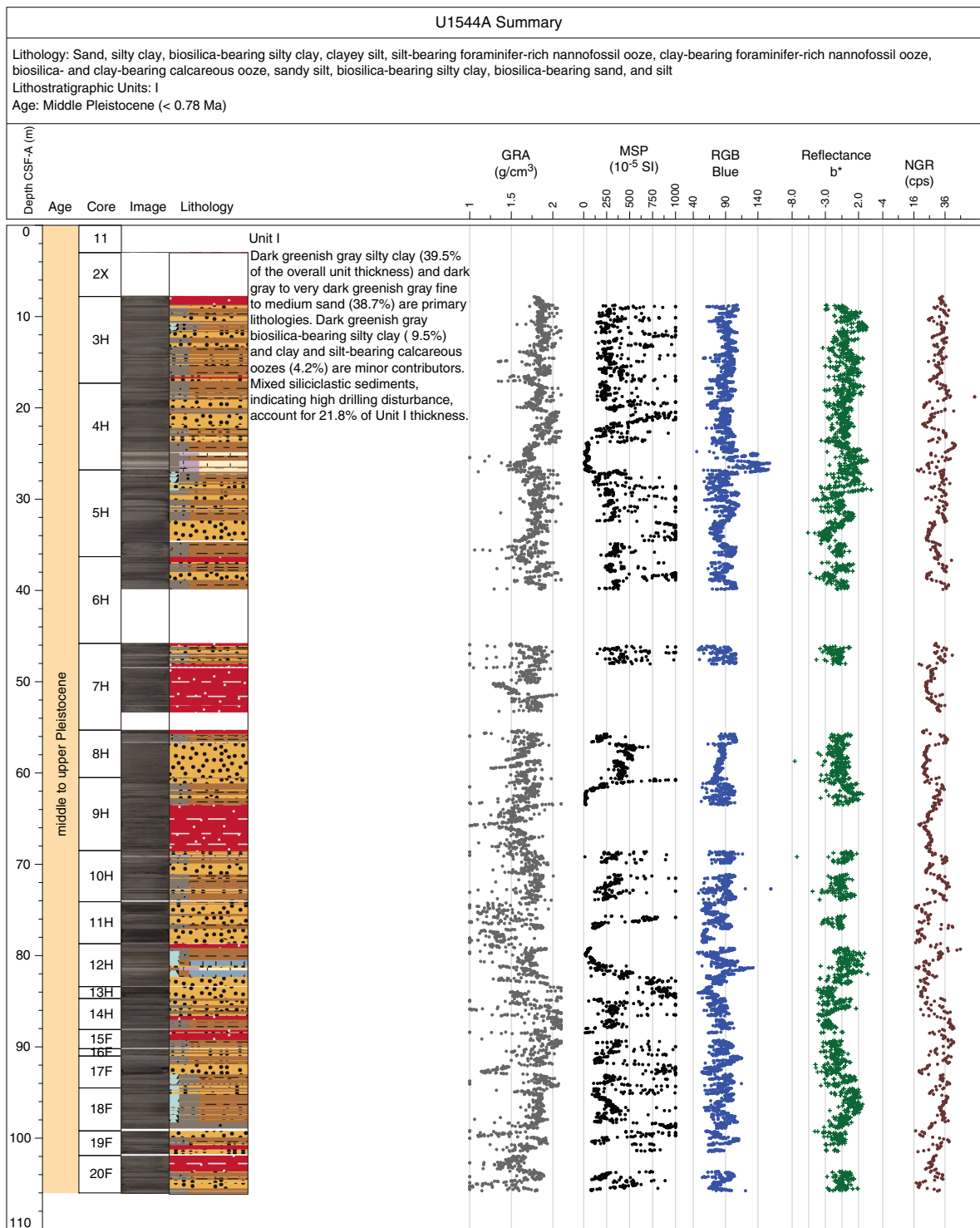
Figure F53. Hole summary, Site U1544. GRA = gamma ray attenuation bulk density, MSP = point magnetic susceptibility, RGB = red-green-blue, NGR = natural gamma radiation, cps = counts per second.
