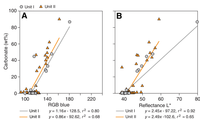
Figure F48. Relationships between bulk sedimentary carbonate content and (A) red-green-blue (RGB) blue and (B) color reflectance L*, Hole U1543A.
