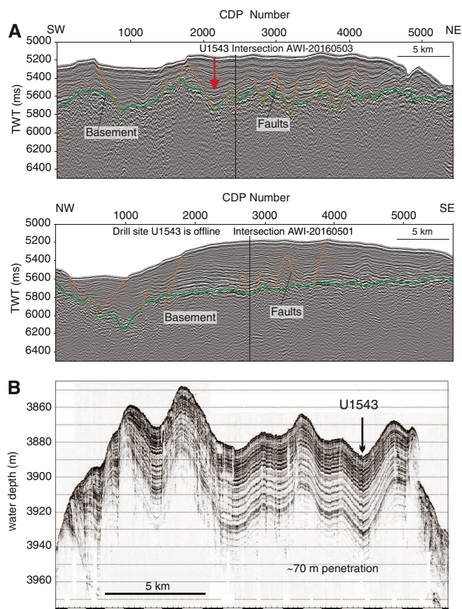
Figure F44. (A) Multichannel seismic (MCS) and (B) Parasound profiles, Site U1543. TWT = two-way traveltime, CDP = common depth point.
