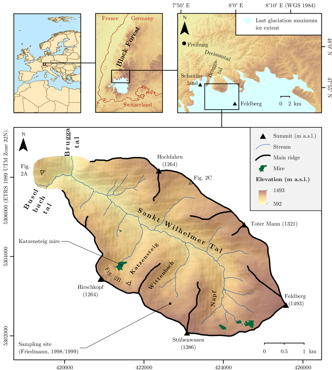
Figure 1. Map of the study area showing mires, the locations where photos were taken for Fig. 2 and localities mentioned in the text. The last glacial maximum extent in the southern Black Forest is highlighted in light blue (Hemmerle et al. , 2016). The shaded relief in the background was derived from a digital terrain model obtained during the SRTM (NASA Jet Propulsion Laboratory, 2013). © EuroGeographics for the administrative boundaries. [Color figure can be viewed at wileyonlinelibrary.com ]
