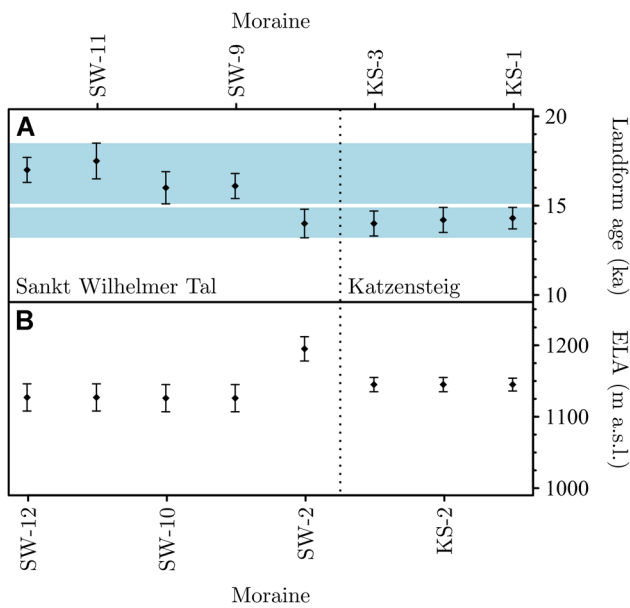
Figure 7. (A) 10 Be CRE ages of moraines and (B) ELAs during their formation. The landform ages indicate two phases of glacial re-advances and/or standstills during deglaciation of the study area (highlighted in light blue). [Color figure can be viewed at wileyonlinelibrary.com ]
