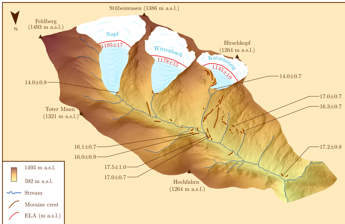
Figure 6. Moraines, glaciers and equilibrium line altitudes (ELAs) in the study area at around 14 ka. 10 Be CRE ages of moraines are presented in ka (thousand years before 2010 CE). [Color figure can be viewed at wileyonlinelibrary.com ]
