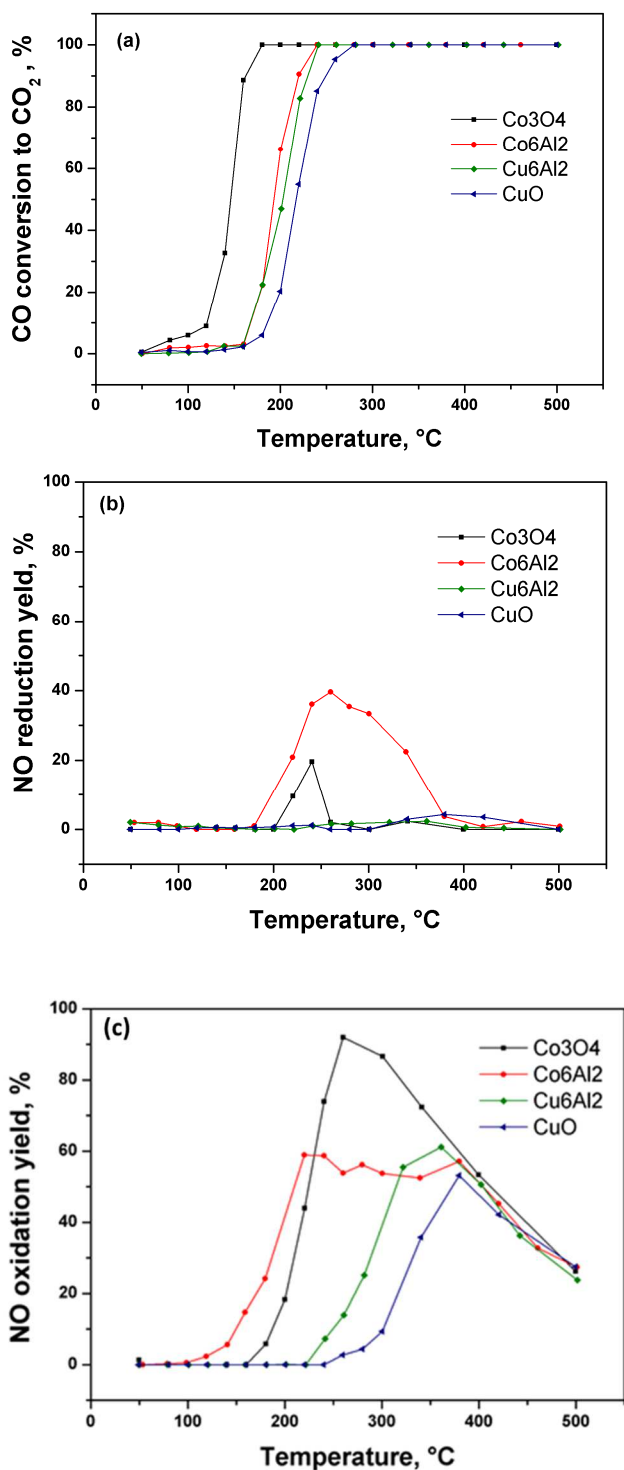
Figure 8. Catalytic results obtained for the different calcined oxide catalysts: (a) CO oxidation to CO 2 ; (b) NO reduction yield; (c) NO oxidation yield. Reaction performed without water added to the feed.
