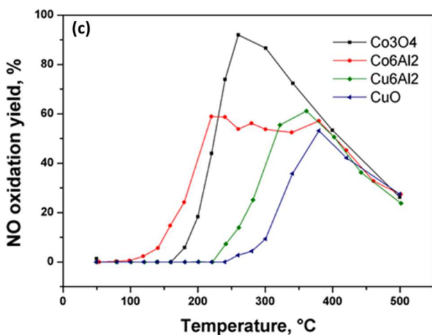
Figure 8. Catalytic results obtained for the different calcined oxide catalysts: (a) CO oxidation to CO 2 ; (b) NO reduction yield; (c) NO oxidation yield. Reaction performed without water added to the feed.
