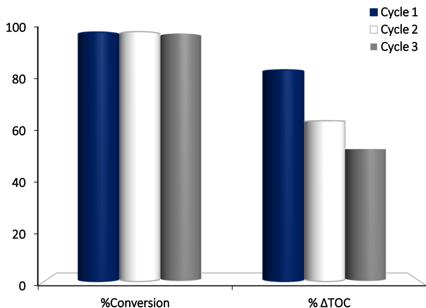
Fig. 8 Catalytic performance of Fe/NiP reused three times in consecutive CWAO reactions. Conversion of BPA and TOC abatement ( \Delta TOC) after 180 min of reaction.
