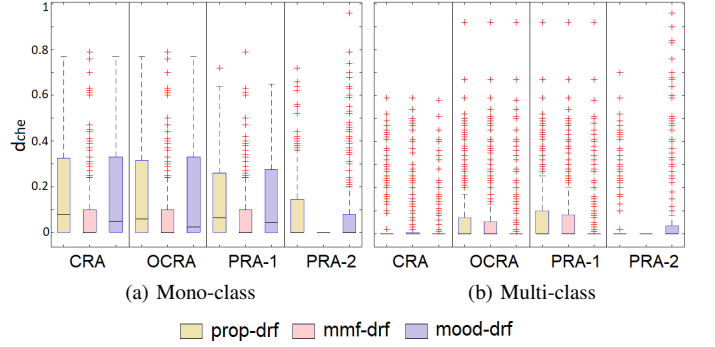
Fig. 10: Chebyshev distance.
