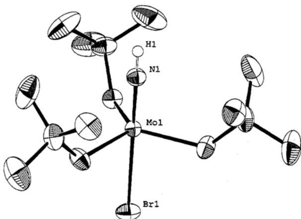
Figure 2. PLATON diagram for compound 4c . Selected structural parameters are as follows: Mo–Br, 2.687(1) Å; Mo–N, 1.692(3) Å; Mo–C (average), 2.110(4) Å; N–H, 0.84(4) Å; Br...H, 2.53(4) Å; Br–Mo–N, 179.41(9)°; Mo–N–H, 179.5(26)°.
