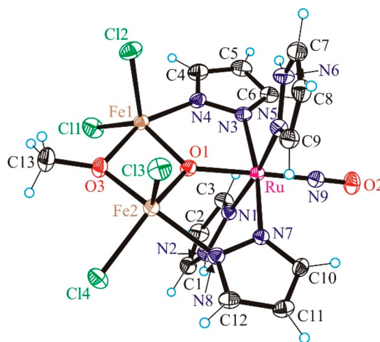
Figure 2. ORTEP view of [\text{Fe}_2\text{RuCl}_4(\mu_3\text{-O})(\mu\text{-OMe})(\mu\text{-pz})_2(\text{NO})(\text{Hpz})_2] ( 6 ). Selected bond distances (Å) and bond angles (deg): Ru–O1 1.9459(19), Ru–N9 1.758(3), Ru–N1 2.076(2), Ru–N3 2.063(2), Ru–N5 2.071(2), Ru–N7 2.068(2), Fe1–O1 1.931(2), Fe1–O3 1.992(2), Fe1–N4 2.076(3), Fe1–Cl1 2.2411(9), Fe1–Cl2 2.2408(9), Fe2–O1 1.950(2), Fe2–O3 1.960(2), Fe2–N8 2.082(2), Fe2–Cl3 2.2200(9), Fe2–Cl4 2.2639(8), N9–O2 1.146(3); N9–Ru–O1 176.92(10), O2–N9–Ru 176.0(2).
