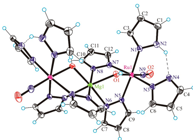
Figure 1. Structure of \{[\text{Ru}(\mu\text{-OH})(\mu\text{-pz})_2(\text{pz})(\text{NO})(\text{Hpz})]_2\text{Mg}\} ( 4 ). Selected bond distances (Å) and bond angles (deg): Ru1–O1 1.9672(12), Ru1–N9 1.7428(16), Ru–N1 2.0873(15), Ru–N3 2.0608(14), Ru–N5 2.0495(15), Ru–N7 2.0772(14), Ru1...Mg 3.37114(17), Mg–O1 2.0347(12), Mg–N6 2.1712(15), Mg–N8 2.1622(14), N9–O2 1.150(2); N9–Ru–O1 176.48(6), O2–N9–Ru 178.05(16).
