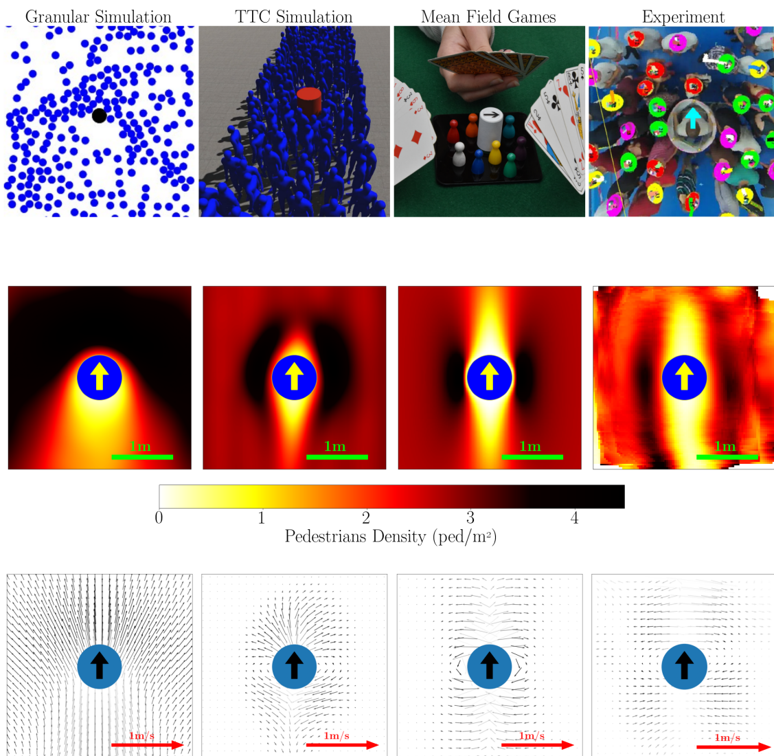
FIGURE 1: Density (middle row) and velocity (bottom row) fields induced in a static crowd by a cylindrical intruder that crosses it; the transparency of the velocity arrows is linearly related to the local density. (Column 1) Simulations of a mono-layer of vibrated disks. (Column 2) Simulations of an agent-based model a wherein agents may anticipate the most imminent collision. (Column 3) Results of the mean-field game introduced in this paper. (Column 4) Controlled experiments of [15]. Note the relatively symmetrical density dip in front and behind the intruder, as well as the transverse moves. (Columns 1-3) The crowd’s density and intruder’s size have been adjusted to match the experimental data. Details of simulations and videos showcasing time evolution can be found in SI.
