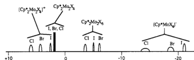
Figure 1. Approximate position and line width for the ^1\text{H-NMR} resonances of all \text{Cp}^* species described in this paper. For comparison, the resonances of the previously reported 9 analogous Cl complexes are also shown.
