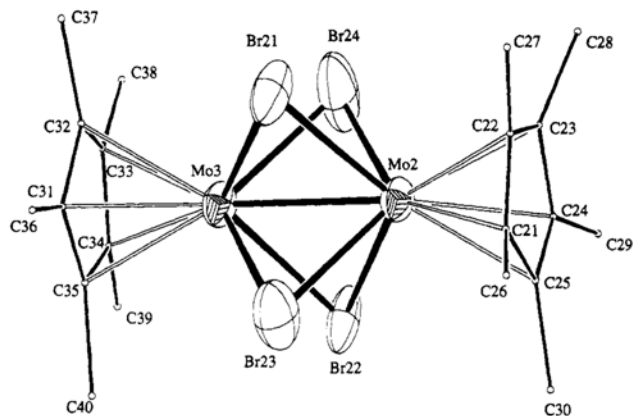
Figure 3. ORTEP view of the [\text{Cp}^*_2\text{Mo}_2\text{Br}_4]^+ ion in compound \{[\text{Cp}^*_2\text{Mo}_2\text{Br}_4]^+[\text{Cp}^*\text{MoBr}_4]_2\}_2\cdot\text{Cp}^*\text{MoBr}_4 . Ellipsoids are drawn at the 40% probability level. Hydrogen atoms are omitted and carbon atoms are drawn with arbitrary radii for clarity. The geometry of the molecule is identical to that observed for the corresponding neutral species, \text{Cp}^*_2\text{Mo}_2\text{Br}_4 , a view of which is available in our preliminary communication. 12
