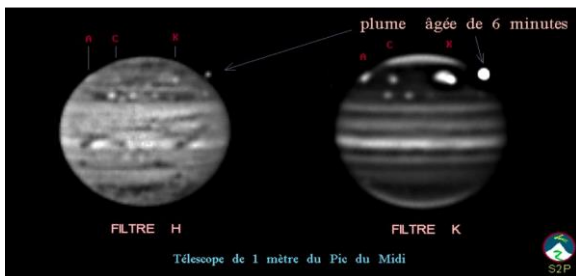
Figure 3 : Impacts of SL9 comet on Jupiter. On the right image, made with CH4 narrow band filter, it is
