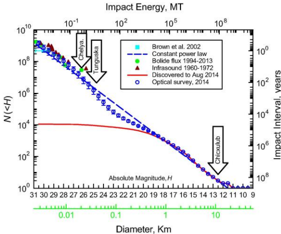
Figure 2 : Cumulative distribution of Near Earth Asteroids (Harris and D'Abramo, 2015)
