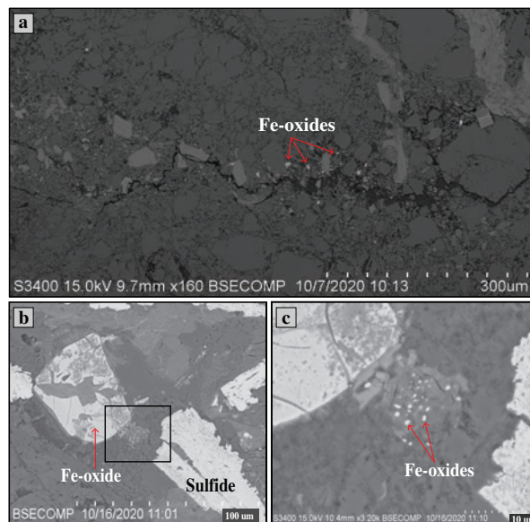
Figure 2: BSE image of a) granitoid sample 1216.97 mbsf and b,c) dolerite sample 939.08. Black square outline in b) shows the enlarged area in image c).
