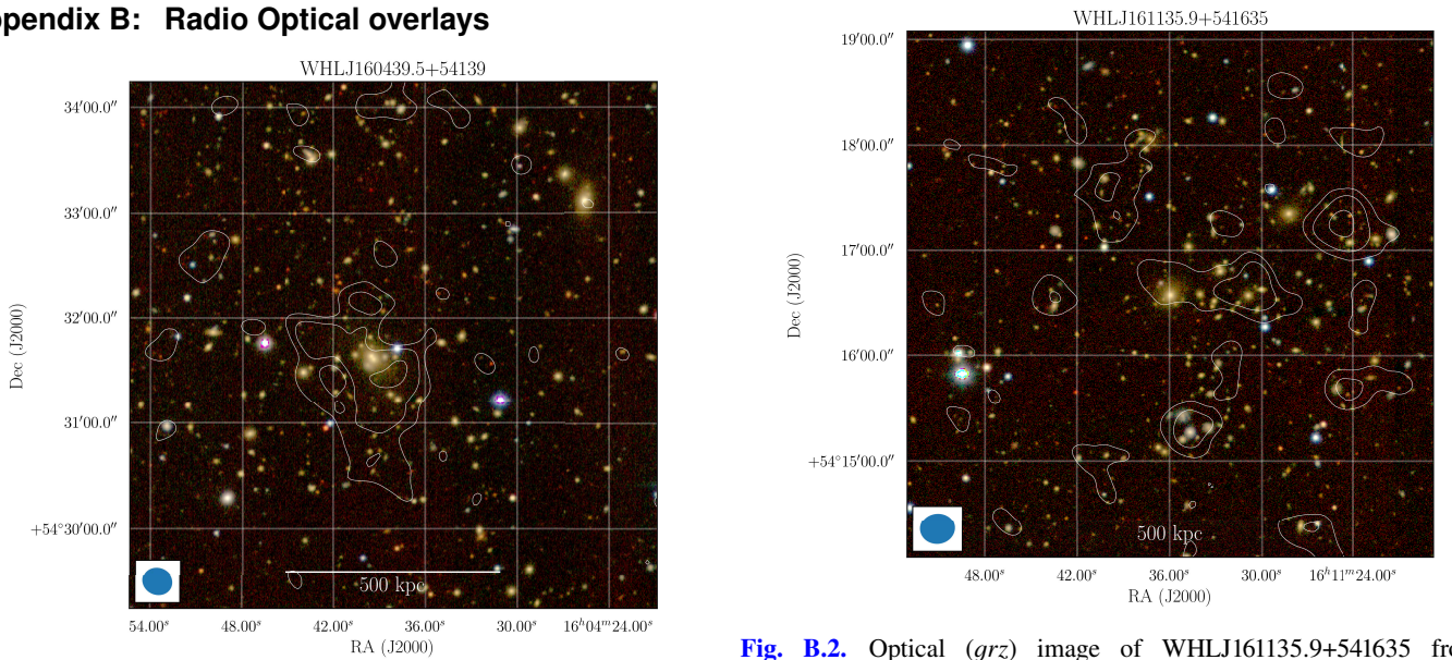
Fig. B.1. Optical ( grz ) image of WHLJ160439.5+54139 from the Legacy Survey with compact source subtracted low-resolution LOFAR contours overlaid. The beam size is 17'' \times 15'' . Contours at [3, 6, 12, \dots]\sigma , where \sigma = 72 \mu\text{Jy beam}^{-1} .
