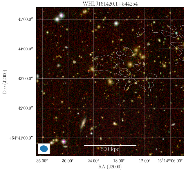
Fig. B.3. Optical ( grz ) image of WHLJ161420.1+544254 from the Legacy Survey with compact source subtracted low-resolution LOFAR contours overlaid. The beam size is X16 \times 13'' . Contours at [3, 6, 12, \dots]\sigma , where \sigma = 66 \mu\text{Jy beam}^{-1} .
