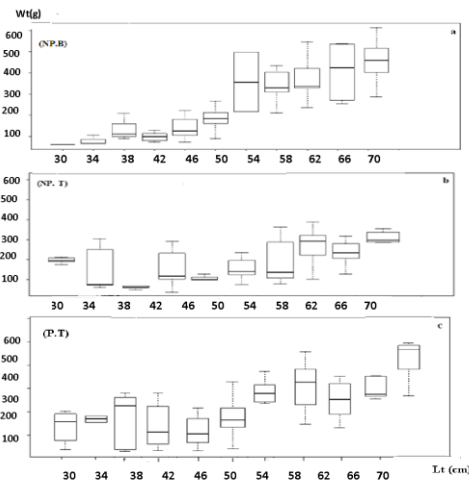
Figure 4. — Weight variations in terms of size-class for the three eel populations at the two stations. PT: Lake Tonga parasitized, NPT: Lake Tonga none parasitized, NP.B: Bou Haroun ports none parasitized.
