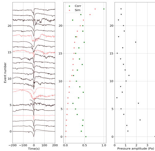
Figure D4. Pressure cluster 2: aligned waveforms. Same as D3 but for cluster 2.
