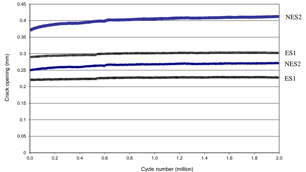
Figure 9. Evolution of crack opening extremes during fatigue tests of NES2 and ES1.
