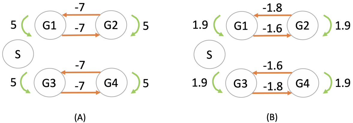
Figure 6: Inference of a 4-genes network (G1 to G4) consisting in two independent symmetric toggle-switch networks with parameters described in Table 1. The stimulus (S) has no effect on the network, but is nevertheless represented in order to verify whether the inferred network takes it into account or not. The network used for simulating the datasets in (A) is compared with the network inferred by CARDAMOM in (B).
