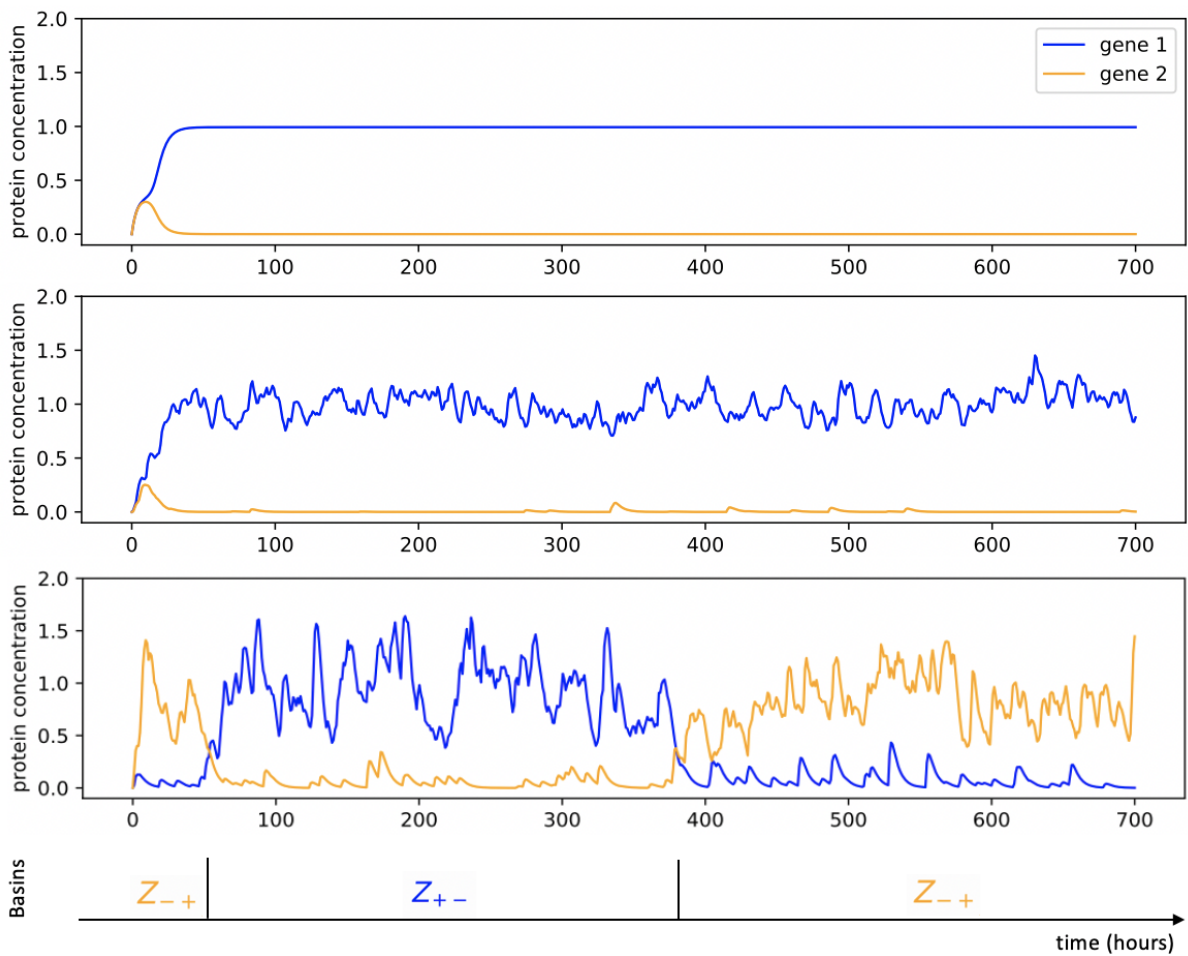
Figure 2: Example of trajectories associated to the symmetric toggle-switch network described in Table 1, for different values of \varepsilon : from top to bottom, \varepsilon = 0 , \varepsilon = 1/50 and \varepsilon = 1/10 . For \varepsilon = 1/10 , we observe stochastic transitions between the two metastable basins denoted Z_{+-} and Z_{-+} .
