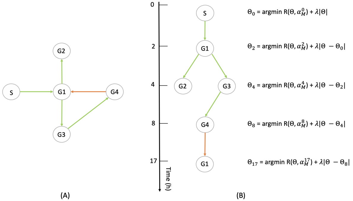
Figure 5: (A) Example of a 4-genes network (G1 to G4) with a stimulus (S) (see Section 5.1). (B) Illustration of the method described in Section 4.2.2: the interactions being observable only at some particular timepoints, they are progressively inferred, each optimization taking into accounts the interactions that are observed on the previous ones.
