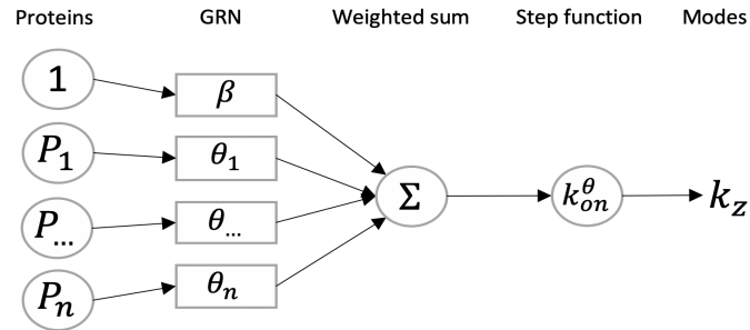
Figure 13: CARDAMOM can be interpreted as the learning of a perceptron, where the clustering step (Section 4.2.1) corresponds to the classification of the data, regarding to their associated modes of frequency, and the regression step (Section 4.2.2) to the identification of the weights of the perceptron, corresponding to the GRN.
