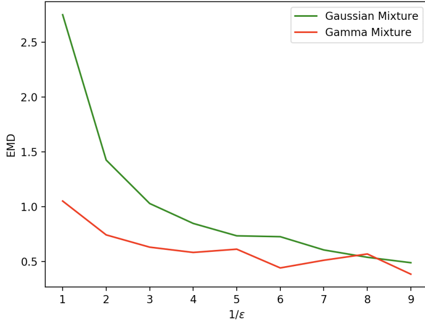
Figure 3: Evolution in function of 1/\varepsilon of the Wasserstein distances between the empirical distribution associated to a set of 2000 cells, simulated with the model (3), and both the Gamma mixture approximation (6) (in red) and a GMM approximation (in green), for the toggle-switch network described in Table 1.
