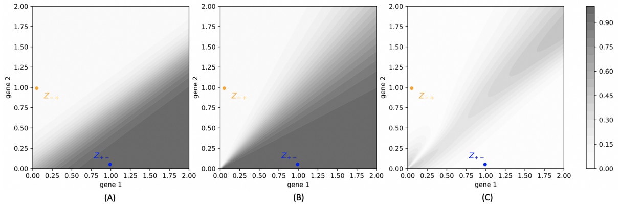
Figure 14: (A): Color map of the function k_{on,1}^\theta/k_{1,1} characterized by the toggle-switch described in Table 1, on the gene expression space. (B): Color map of the function k_{on,1}^\alpha/k_{1,1} characterized by the mixture parameters associated to the same network, obtained with the method described in Figure 4, on the gene expression space. (C): Color map of the function |k_{on,1}^\theta - k_{on,1}^\alpha|/k_{1,1} , on the gene expression space.
