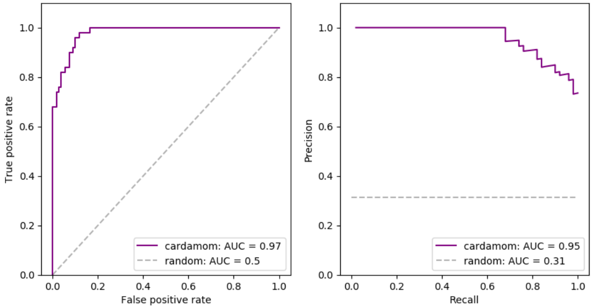
Figure 7: Inference results for the 4-gene network described in Table 2. Performances are measured in terms of receiver operating characteristic curves (ROC) and precision-recall curves (PR) obtained for 10 independently simulated datasets. Each dataset contained the same 10 timepoints and 50 cells per time point. The dashed gray line indicates the average score that would be obtained by the random estimator (detecting a link or not with equal probability).
