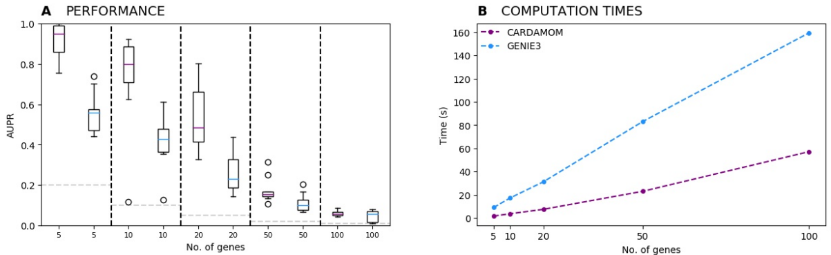
Figure 11: (A) Evolution of the performances of CARDAMOM and GENIE3 when increasing the number of genes. For each number of genes, we represent a boxplot of the AUPR scores computed for ten datasets simulated with 10 different randomly generated tree-like networks. (B) Evolution of the average computational time measured for inferring the tree-like networks with respect to the number of genes.
