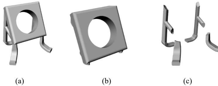
Figure 14 – (a). The CAD model of case 2; (b). The initial volume; (c). The remaining volumes to deposit material onto the initial volume.
