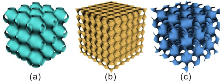
Fig. 4. Different types of TPMS structures (3*3): (a). Schwarz Primitive surface; (b). Schwarz Diamond surface; (c). Schoen Gyroid surface.
