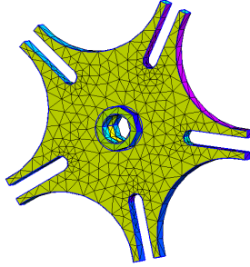
Figure 6: Tetrahedral mesh of a Geneva wheel.
