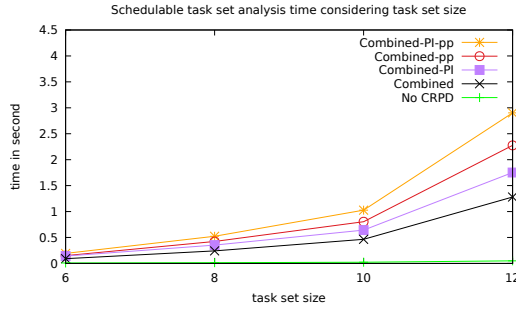
Figure 6: Analysis time for a cache memory of 4KB, 2 ways, U = 0.85 , BRT = 200 and M_{reduce} = 4
