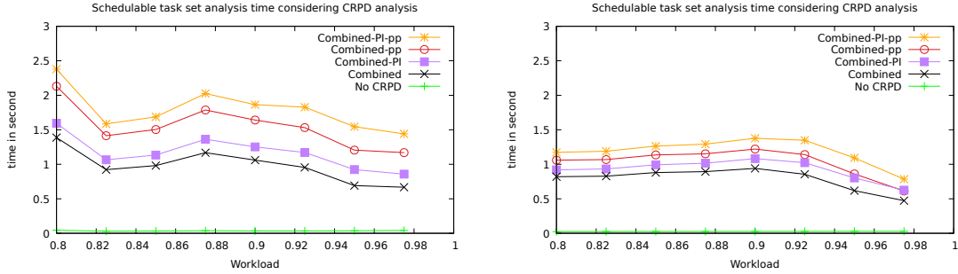
(a) Analysis time for n_{tasks} = 12 with cache memory of 2KB, 4 ways, BRT = 50 and M_{reduce} = 4 (b) Analysis time for n_{tasks} = 12 with cache memory of 2KB, 4 ways, BRT = 50 and M_{reduce} = 2
