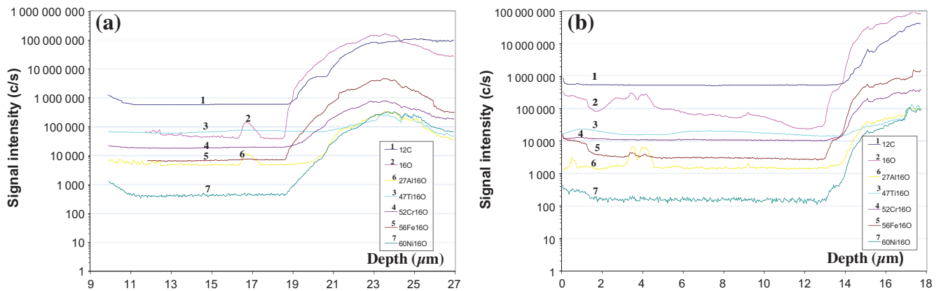
Fig. 9. Composition profile of elements ( ^{16}\text{O} , ^{12}\text{C} ) and oxides ( ^{16}\text{OTi} , ^{16}\text{OCr} , ^{16}\text{ONi} ) versus depth (from base metal (left side) to the oxide layer) obtained by reverse SIMS for (a) polished sample exposed to PWR environment and (b) ground sample exposed to PWR environment (circled highlights showing the presence of aluminum oxides dispersed in the metal matrix) – a deeper depth has been studied in the metal for (a) than for (b).
