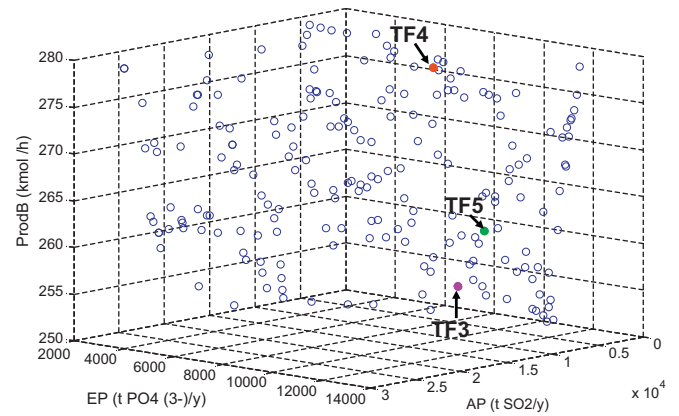
Fig. 12. Triobjective optimization (ProdB, EP, AP) – Case 2.
