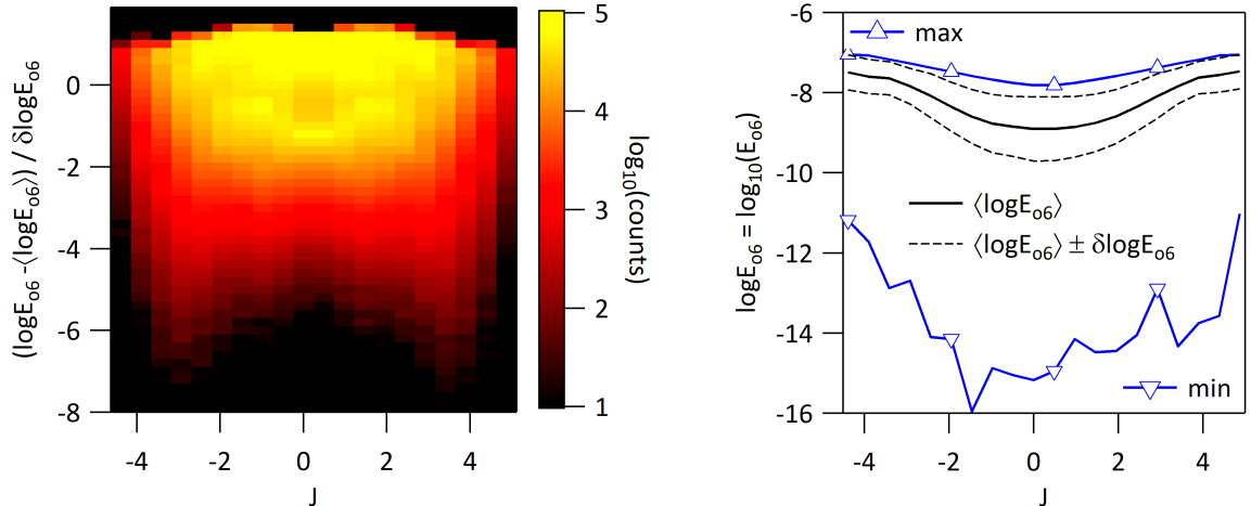
Figure 14: PoPe error for case a , \sigma_{chir} = 7.0 and \nu = 0.2 , RK4 integration with N = 2^8 points per unit time, reconstruction with finite difference of order 6. Left hand side: Histograms for different values of J and normalised statistics. Right hand side, variation of the mean \langle \log E_{o6} \rangle , max and min of \log E_{o6} as well as the characteristic width of the distribution function determined by the standard deviation \delta \log E_{o6} , namely \langle \log E_{o6} \rangle \pm \delta \log E_{o6} .
