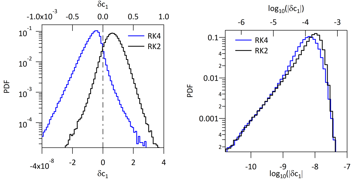
Figure 42: PDF to compare data from RK2 simulation, top scale black PDF, and data from RK4 simulation, bottom scale blue PDF. Left hand side: PDF of \delta c_1 . Right hand side : PDF of \log_{10}(|\delta c_1|) . All simulations of case a with time step 1/2^9 and setting c_4 = 0 in the PoPe analysis.
