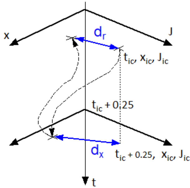
Figure 4: Verification with the Method of Return Solution, sketch of the method.
