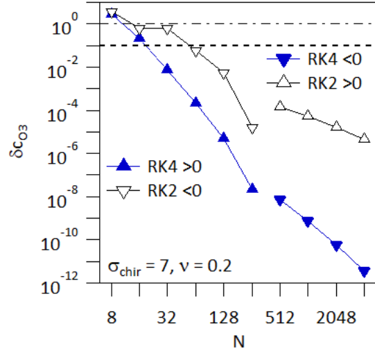
Figure 29: Sign and scaling law of the PoPe projection of the error \delta c_{O_3} for given integration scheme, RK4 closed blue triangles, and RK2 open black triangles, versus the number of steps per unit time N for case a , \sigma_{chir} = 7 , \nu = 0.2 . Head-up triangles positive absolute error, head-down triangles negative absolute error.
