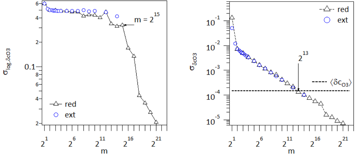
Figure 21: Effect of the number of m -tuples on the standard deviation \sigma with the extended statistics, ext blue open circles, and reduced statistics, red black triangles for the operator O_3 . Left hand side: Statistics on \log_{10}(|\delta c_{O_3}|) , standard deviation \sigma_{\log, \delta c_{O_3}} versus m . The transition from near constant standard deviation to roughly an exponential decrease occurs for m \approx 2^{15} . Right hand side: Statistics on \delta c_{O_3} , standard deviation \sigma_{\delta c_{O_3}} versus m . The asymptotic value of the mean \langle \delta c_{O_3} \rangle is plotted with a dashed black line. The standard deviation becomes smaller than the mean value, \sigma_{\delta c_{O_3}} / \langle \delta c_{O_3} \rangle \leq 1 , for m \geq 2^{13} .
