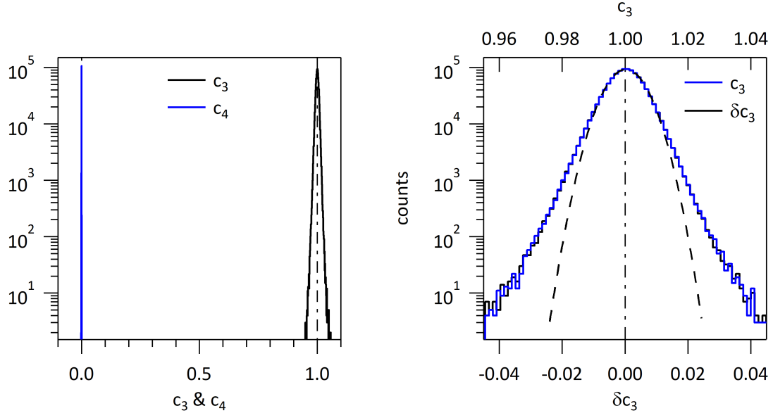
Figure 40: Histogram for case a simulations with RK2 time stepping and time step 1/2^9 . Left hand side : Histogram of coefficients c_3 , black histogram, and c_4 , blue histogram, computed with E_{O_3} , Eq.( 38a). Right hand side: top scale, blue histogram coefficient c_3 computed with the error E_{O_3} , Eq.( 38a), lower scale, black histogram, coefficient \delta c_3 computed with the standard expression of the error Eq.( 37a).
