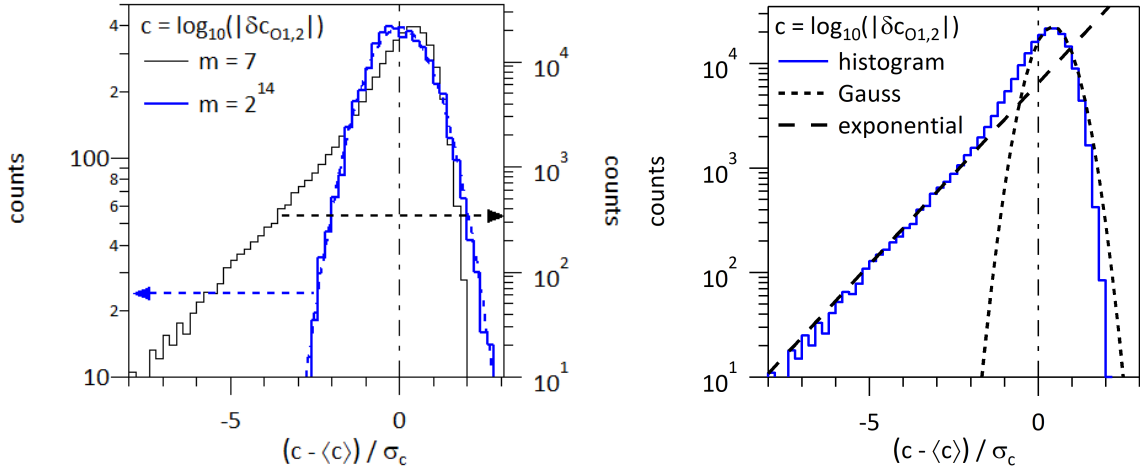
Figure 26: Left hand side: Histograms for m = 2^{14} thick blue line, Gaussian fit dashed blue line, and for m = 7 , black line, versus the normalised variation (c - \langle c \rangle) / \sigma_c for c = \log_{10}(|\delta c_{O1,2}|) . Right hand side: Histogram for m = 7 versus for (c - \langle c \rangle) / \sigma_c for c = \log_{10}(|\delta c_{O1,2}|) as on left hand side, with exponential fit towards the small errors and Gaussian fit for the errors comparable to the mean value.
