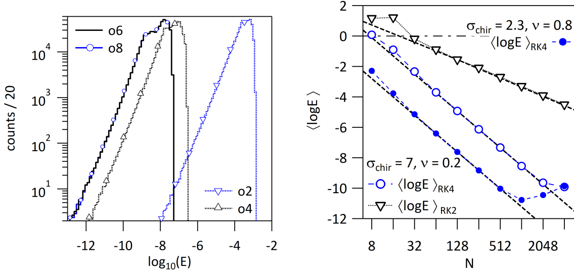
Figure 15: Left hand side: PoPe error for case a \sigma_{chir} = 7 and \nu = 0.2 , RK4 integration with N = 2^8 points per unit time, comparison of the histograms of \log E obtained with finite difference scheme of order 2 head down triangles dashed blue curve, and order 4 head up triangles dashed black curve, order 6 black plain line and order 8 blue plain line open blue circles. Right hand side: variation of the mean error \langle \log E \rangle with the number of steps of the integration scheme for the Runge Kutta schemes of order 2, black curve head down open triangles, and order 4, blue curves with circles and for the control parameters of case b , \sigma_{chir} = 2.3 and \nu = 0.8 , closed symbols, and case a , \sigma_{chir} = 7 and \nu = 0.2 open symbols.
