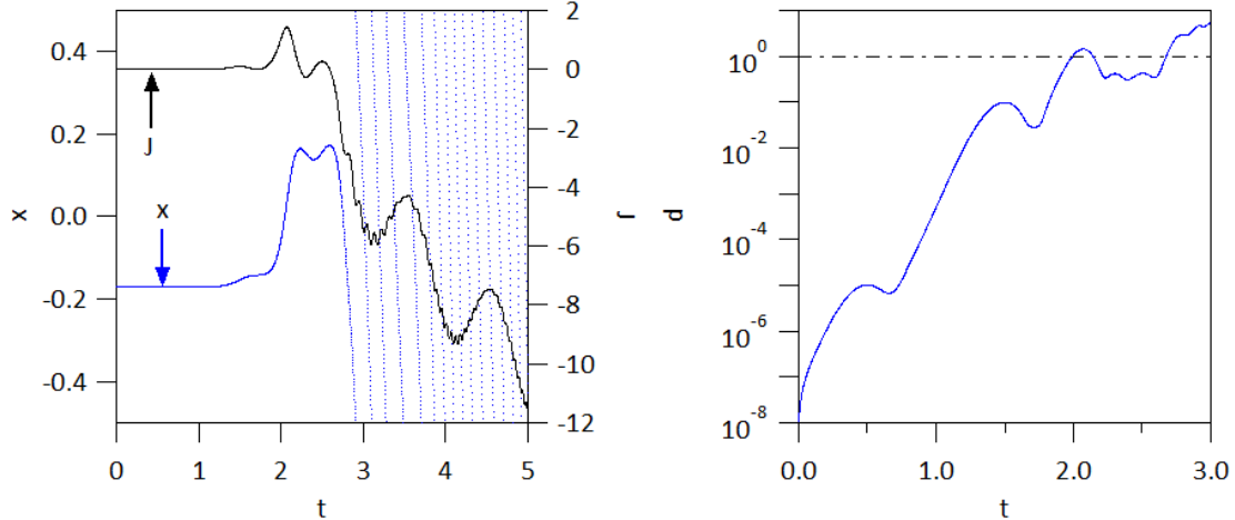
Figure 3: For case a , \sigma_{chir} = 7 and \nu = 0.2 , investigation of the fixed point stability for the standard Method of Manufactured Solution, trajectory with chosen fixed point X = x_0 = -0.17 , J = 0 and initial distance from this fixed point d_0 = 10^{-8} . Left hand side: trace of x (blue dotted curve) and J (black curve). Right hand side: variation of the distance d from the fixed point, initial value d_0 = 10^{-8} with rapid growth to macroscopic values, d \approx 1 on a time scale of \delta t \approx 2 .
