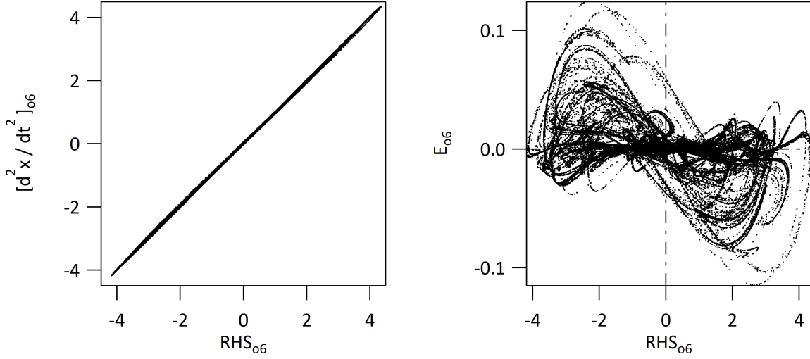
Figure 12: PoPe error for case a \sigma_{chir} = 2.3 , \nu = 0.8 , RK4 integration with N = 2^8 points per unit time, reconstruction with finite difference of order 6. Left hand side: Reconstructed second order derivative of x versus the Right Hand Side (RHS) of Eq.( 24). Right hand side: Error E_{o6} versus the RHS.
