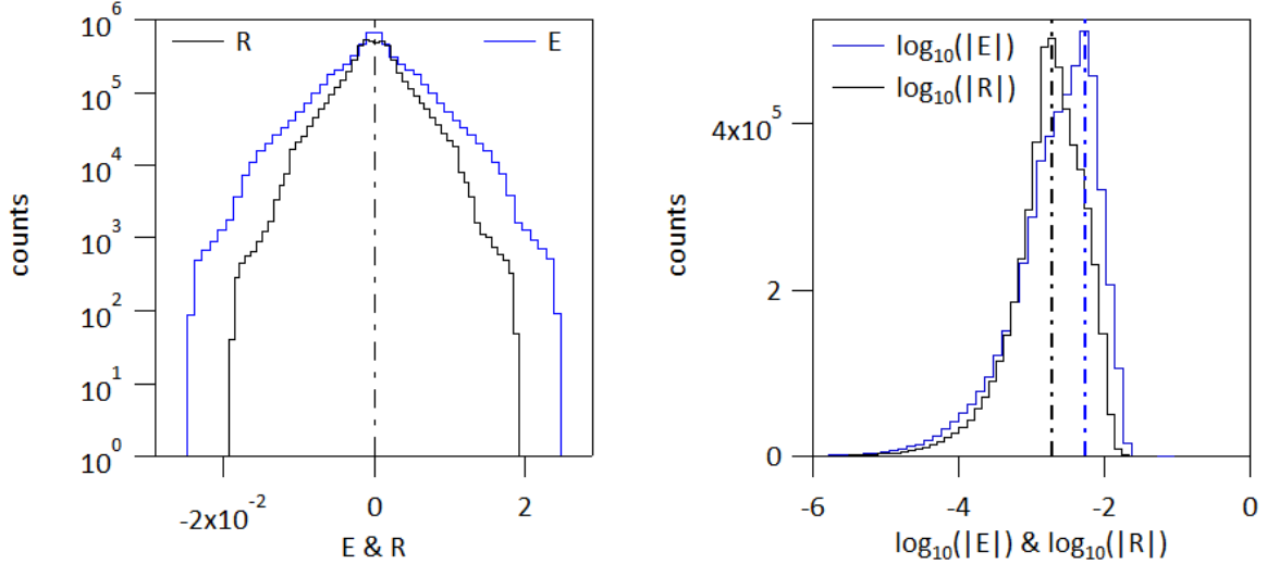
Figure 36: Left hand side: Histograms of the error E , blue line, and residue R , black line. Right hand side: Histograms of \log E = \log_{10}(|E|) , blue line, and \mathcal{R} = \log_{10}(|R|) , black line. The vertical dashed-dot lines for the latter indicate the most probable values. Simulation with RK2 scheme time step 1/N , N = 2^9 .
