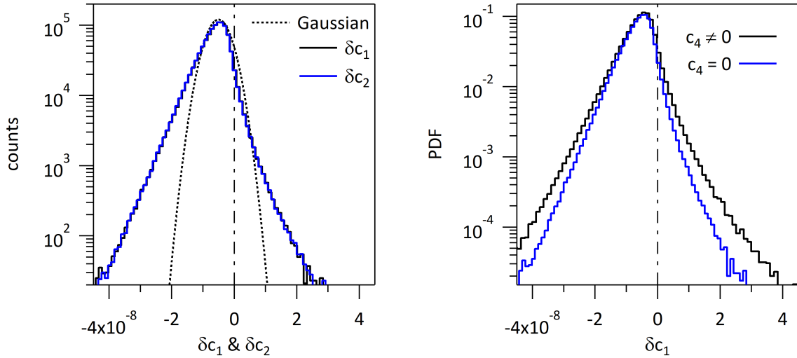
Figure 43: Left hand side: Histograms of \delta c_1 and \delta c_2 setting c_4 = 0 in the PoPe analysis. Right hand side : Histogram of the coefficient \delta c_1 , blue histogram setting c_4 = 0 and when determining c_4 with PoPe, black histogram. All simulations of case a with RK4 and time step 1/2^9 .
