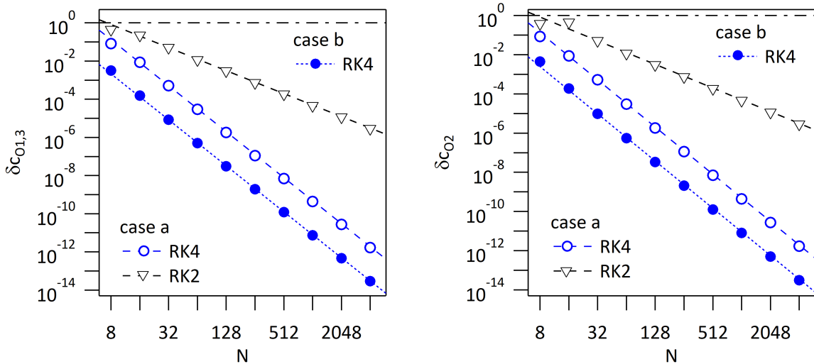
Figure 30: Dependence of the scaling law of the PoPe projection of the error for given integration scheme, RK4 with blue circles and RK2 with black head-down triangles, in terms of the number of steps per unit time N . Left hand side for \delta c_{O_{1,3}} . Right hand side for \delta c_{O_2} . The dashed line are the scaling of the error N^{-4} for RK4 and N^{-2} for RK2.
