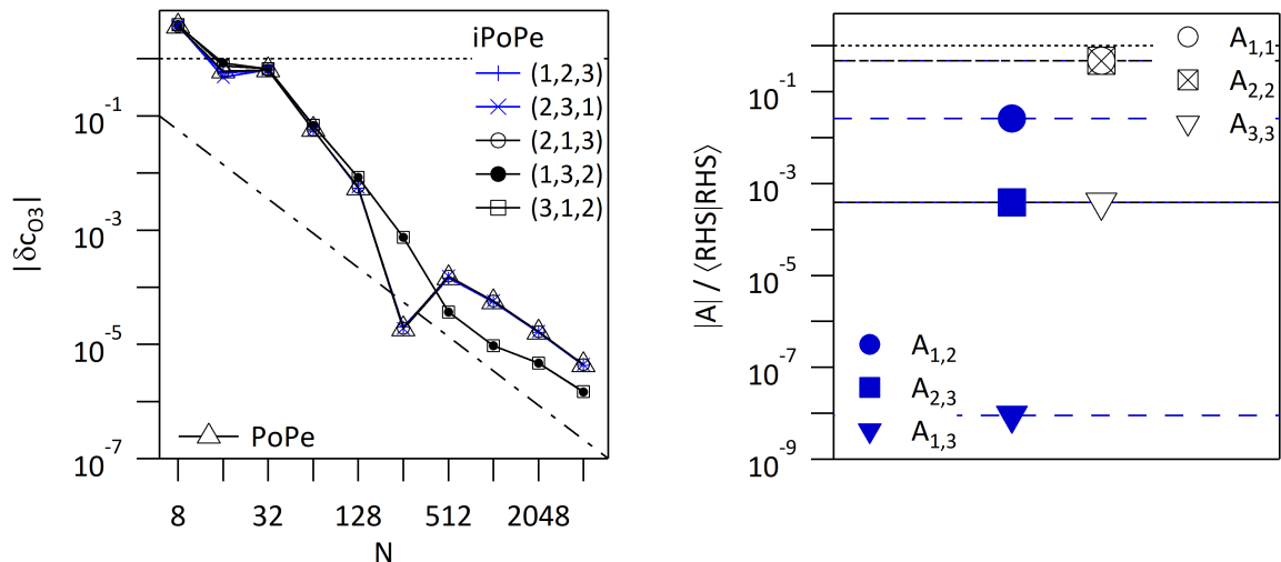
Figure 38: Left hand side: Determination of the coefficients \delta c_{O_3} with both PoPe, black open head-up triangles, and iPoPe: (1, 2, 3) blue plus + marker, (2, 3, 1) blue cross \times marker, (1, 3, 2) black closed circle, (3, 1, 2) black open square, (2, 1, 3) black open circle, (3, 2, 1) black open head down triangle. The dotted line indicates the relative error equal to 1. Right hand side: Values of the symmetric matrix \mathcal{A} / \langle RHS|RHS \rangle , see Table 1, open symbols diagonal elements, closed symbols off-diagonal elements, RK2 simulation of case a with N = 2^9 . The dotted line indicates the value of the sum of all the matrix elements, equal to one for the normalisation by \langle RHS|RHS \rangle .
