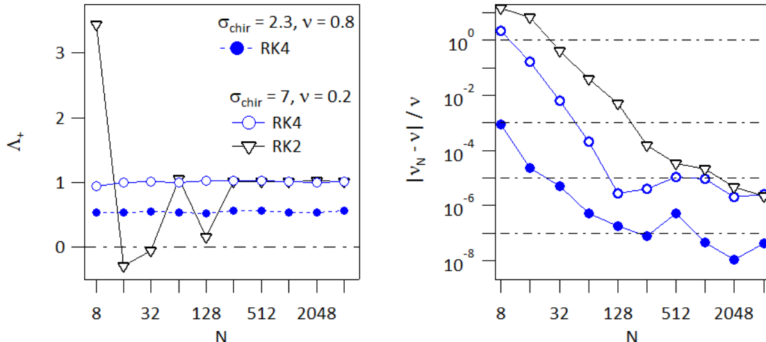
Figure 9: Accuracy investigation for the cases a , \sigma_{chir} = 7, \nu = 0.2 , open symbols, and b , \sigma_{chir} = 2.3, \nu = 0.8 closed symbol with the RK4 and RK2 integration schemes, circles, respectively head down triangles. Left hand side, calculation of the largest Lyapunov exponent \Lambda_+ . Right hand side, relative error on the value of \nu determined by the calculation of the rate of decrease of the phase space volume.
