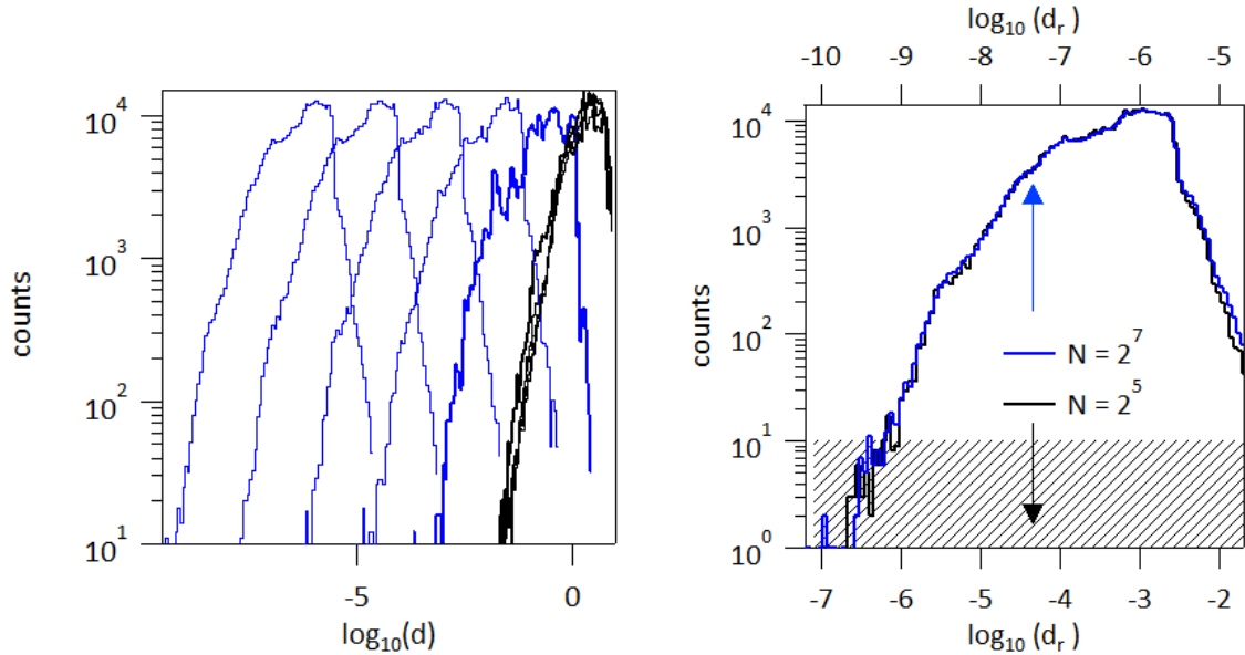
Figure 6: Verification with the Method of Return Solution for case a , \sigma_{chir} = 7 and \nu = 0.2 . Left hand side: histograms of \log_{10}(d) for various resolutions N , N = 2^3, 2^4, 2^5, 2^6, 2^7 , black histograms of d_x black curves, histograms of d_r blue curves. Right hand side: similarity of the MRS error histograms of \log_{10}(d_r) for N = 2^5 lower scale and N = 2^7 upper scale.
