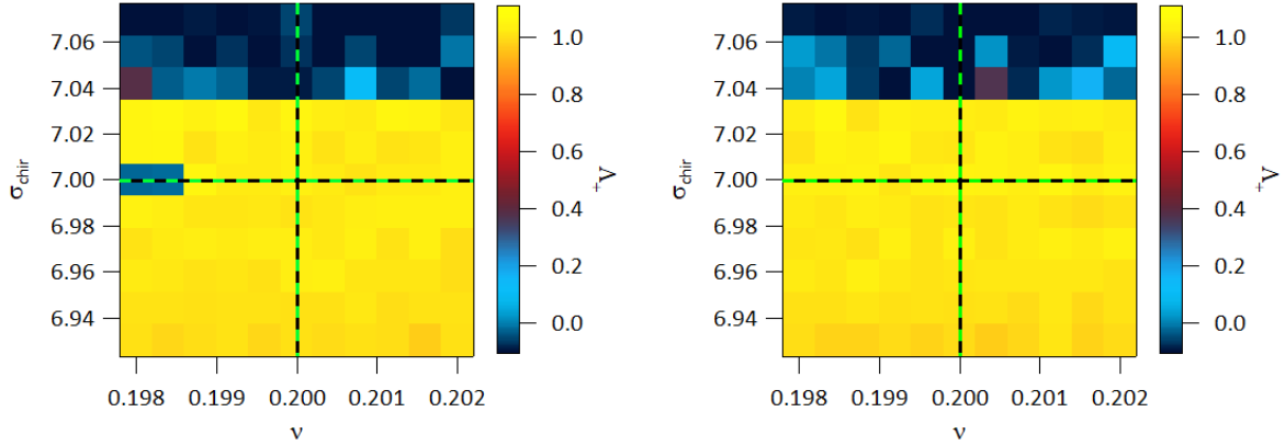
Figure 33: Control parameter space in the vicinity of (\nu_{ref} = 0.2, \sigma_{chir,ref} = 7) with \pm 1\% variation and 11 points in each direction. Each simulation is characterised by the largest Lyapunov exponent \Lambda_+ . Left hand side: Phase portrait for N = 2^8 steps per unit time and RK2 time stepping. Right hand side: Phase portrait for N = 2^7 steps per unit time and RK4 time stepping.
