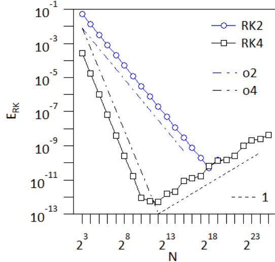
Figure 10: Error E_{RK} obtained with the Manufactured Method Solution for the Runge Kutta schemes, order 2 blue open circles and order 4 black open squares. The corresponding slopes for order 2 and order 4 error are indicated by dash dot lines, respectively blue for order 2 and black for order 4. The dashed black line is indicative of the slope N^1 which fits the loss of accuracy when N is too large.
