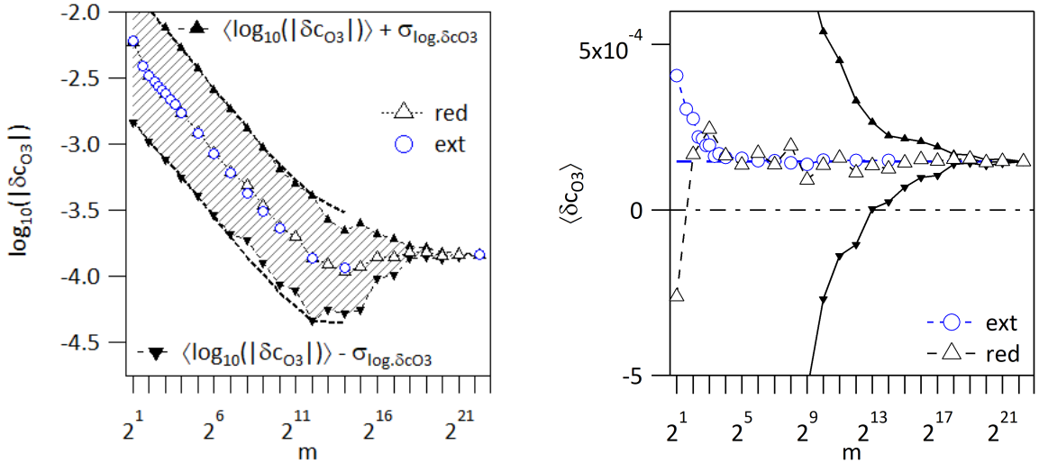
Figure 22: For the operator O_3 , effect of the number of m -tuples on the mean value of the coefficient using the extended statistics, ext blue open circles, and reduced statistics red black triangles. Left hand side: Mean value \langle \log_{10}(|\delta c_{O_3}|) \rangle and region with highest probability between \langle \log_{10}(|\delta c_{O_3}|) \rangle + \sigma_{\log, \delta c_{O_3}} closed head-up triangles, and \langle \log_{10}(|\delta c_{O_3}|) \rangle - \sigma_{\log, \delta c_{O_3}} , closed head-down triangle. Right hand side: Mean value \langle \delta c_{O_3} \rangle and region with highest probability between \langle \delta c_{O_3} \rangle + \sigma_{\delta c_{O_3}} closed head-up triangles, and \langle \delta c_{O_3} \rangle - \sigma_{\delta c_{O_3}} , closed head-down triangle.
