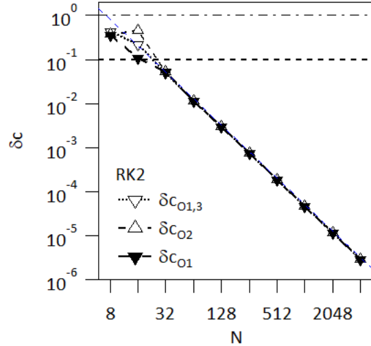
Figure 31: PoPe projection of the error for RK2, coefficients: \delta c_{O1,3} head-down open triangles, \delta c_{O2} head-up open triangles, and \delta c_{O1} head-down closed triangles.
