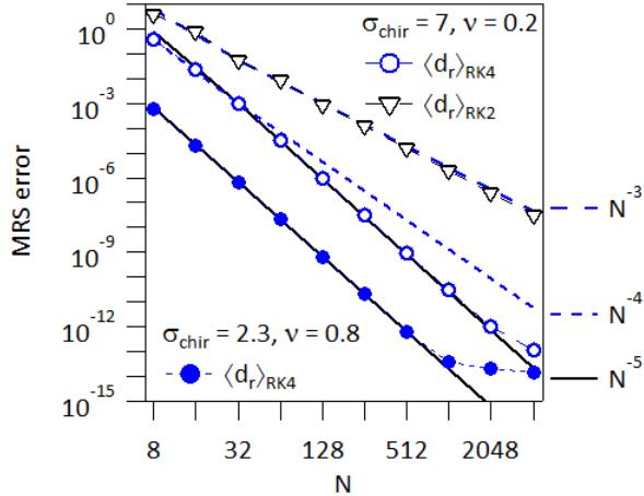
Figure 7: Investigation of the order of the numerical scheme with the Method of Return Solution (MRS). For case a , \sigma_{chir} = 7 and \nu = 0.2 , comparison of the Runge Kutta schemes of order two (RK2), up-down open triangles, and four (RK4) open circles. For case b , \sigma_{chir} = 2.3 and \nu = 0.8 , precision with the Runge Kutta schemes of order four, closed circles. The expected scaling exponents, N^{-5} for RK4 and N^{-3} for RK2, are recovered.
