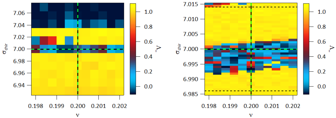
Figure 34: Control parameter space in the vicinity of (\nu_{ref} = 0.2, \sigma_{chir,ref} = 7) with \pm 1\% variation and 11 points in each direction. Each simulation is characterised by the largest Lyapunov exponent \Lambda_+ . Left hand side: Phase portrait for N = 2^7 steps per unit time and RK2 time stepping and different initial conditions. Right hand side: Zoom of the phase portrait for N = 2^7 steps per unit time and RK2 time stepping.
