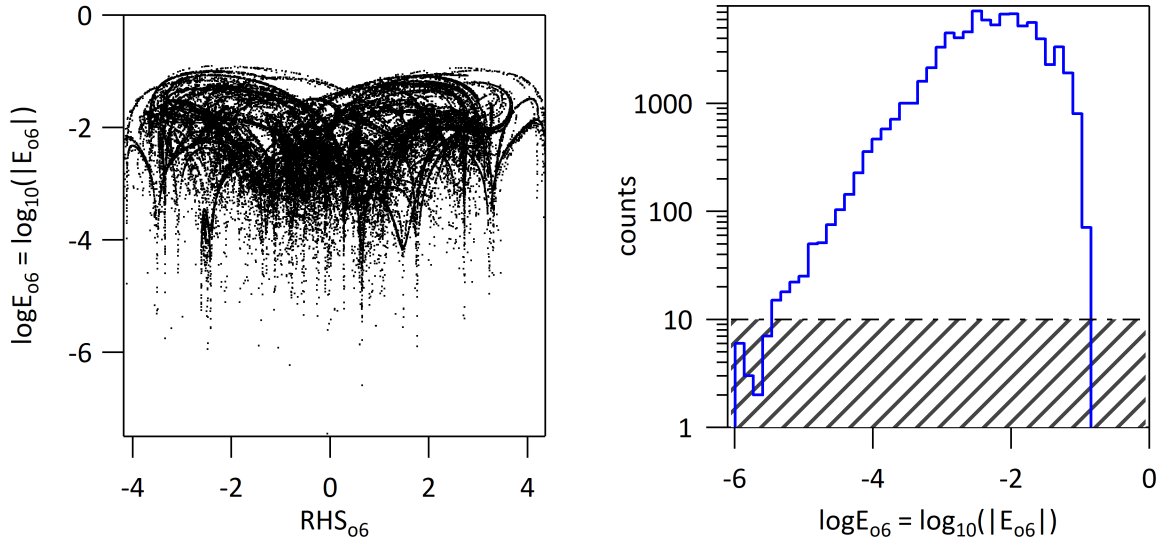
Figure 13: PoPe error for case a , \sigma_{chir} = 2.3 , \nu = 0.8 , RK4 integration with N = 2^8 points per unit time, reconstruction with finite difference of order 6. Left hand side: Left hand side \log_{10}(|E_{o6}|) versus the RHS of Eq.( 24). Right hand side, histogram of this error, the shaded area indicating the region with small statistics and consequent large relative fluctuations. All histograms are build using 5 bins par standard deviation.
