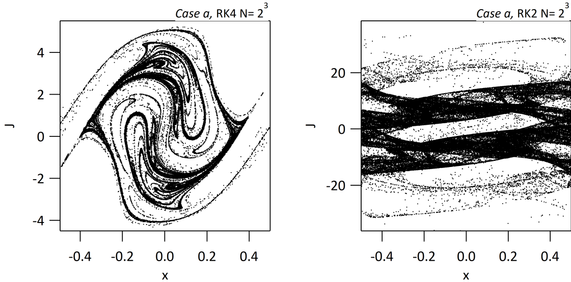
Figure 8: Strange attractor for case a , \sigma_{chir} = 7 , \nu = 0.2 and time stepping with N = 2^3 steps per unit time. Left hand side: fourth order Runge Kutta integration scheme. Right hand side: second order Runge Kutta integration.
