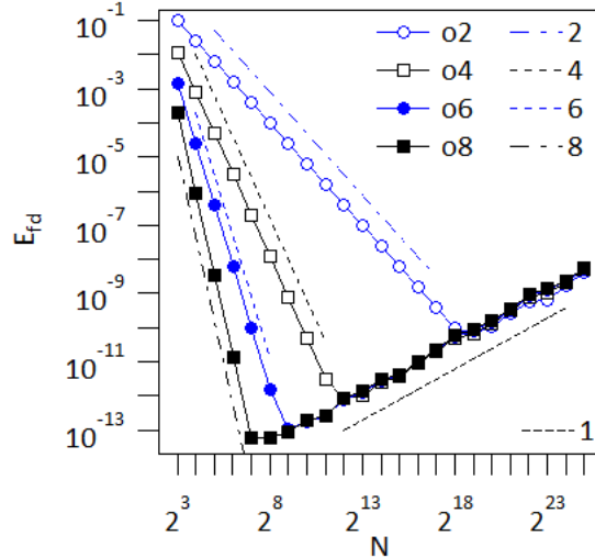
Figure 11: Error E_{fd} obtained by comparing the derivative of \sin(t) to \cos(t) obtained with finite difference, order 2 blue open circles and order 4 black open squares, order 6 blue full circles and order 8, full black squares. The theoretical decay rates are also indicated by the dash dot and dashed lines. The dashed black line with positive slope N^1 fits the loss of accuracy when N is too large.
