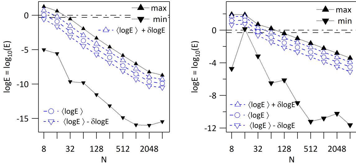
Figure 16: Key features of the histogram of the error \log E , the mean \langle \log E \rangle blue open circles, the mean value plus the standard deviation \langle \log E \rangle + \delta \log E , blue open head-up triangles, the mean value minus the standard deviation \langle \log E \rangle - \delta \log E , blue open head-down triangles, and finally minimum and maximum of the distribution of \log E , respectively head-down full black triangles, and head-up full black triangles. The dashed horizontal line locates \log E \approx -0.3 hence an error E of 50%. Left hand side: case a , \sigma_{chir} = 7 and \nu = 0.2 RK4 integration scheme. Right hand side: case a , \sigma_{chir} = 7 and \nu = 0.2 , RK2 integration scheme.
