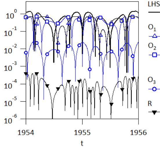
Figure 39: Time trace over 2 periods of the time dependent forcing of the Left Hand Side (LHS) of the evolution equation plain black line and of the three operators that contribute to the right hand side of Eq.( 24), O_1 open blue head-up triangles, O_2 open blue squares, O_3 open blue circles and the residue R , closed black head-down triangle, RK2 simulation of case a , time step 1/N , N = 2^9 . All operators are normalised by the mean plus standard deviation of RHS .
