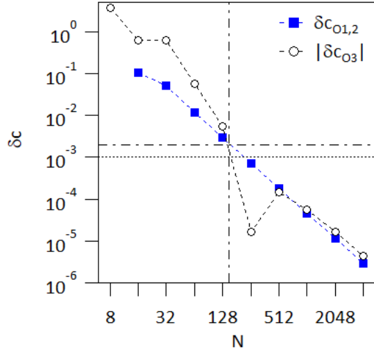
Figure 35: Variation of the relative error determined by PoPe, \delta c_{O_{1,2}} for \sigma_{chir}^2 , closed blue squares, and \delta c_{O_3} for \nu , open black circles. The dashed, respectively dotted line indicates the maximum error for \delta c_{O_3} , respectively \delta c_{O_{1,2}} so that the error is smaller than the mesh size of the phase portrait of Figures 32 and 33.
