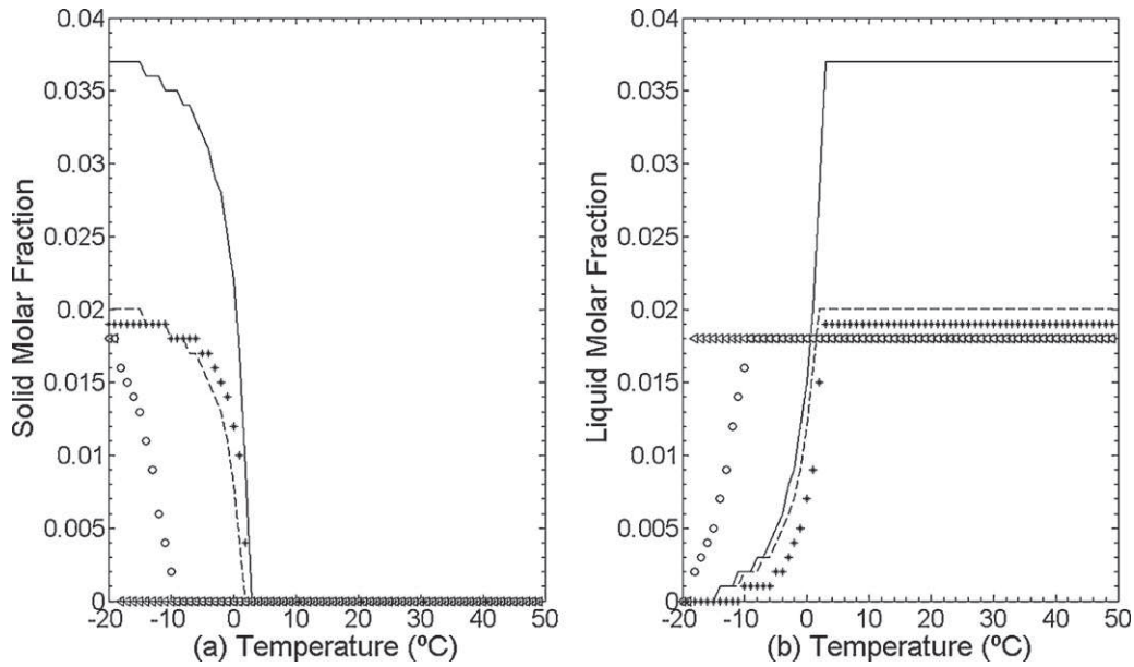
Fig. 4. Molar fraction in the solid phase (a) and liquid phase (b) of palm oil triacylglycerols. POL (—), OPO (---), SOO (***), OOL (°) e OLO (Δ).
