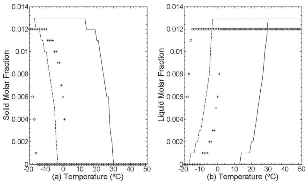
Fig. 5. Molar fraction in the solid phase (a) and liquid phase (b) of palm oil triacylglycerols. PPS (—), PPL (---), PLS (***), PLL (°).
