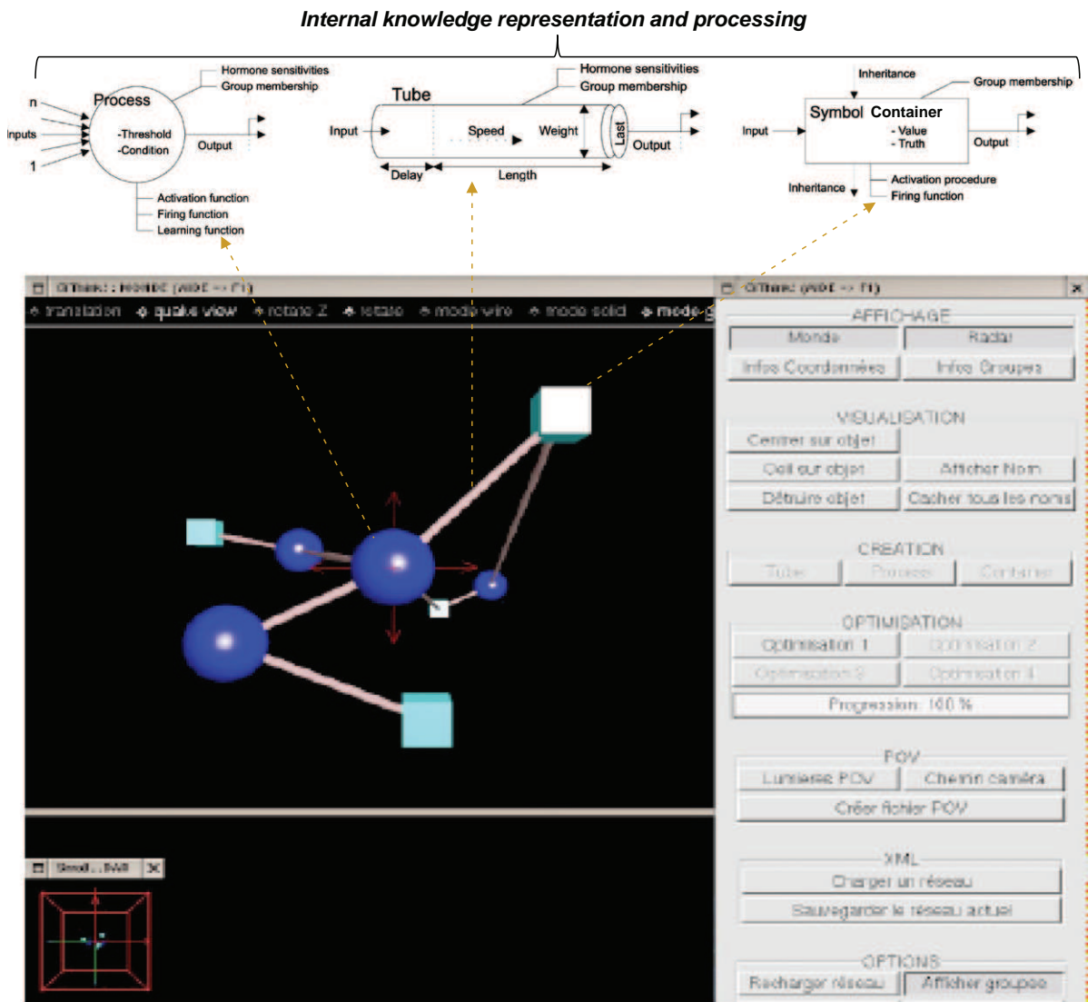
Fig. 3. The 3D visualization of a Think! network.
