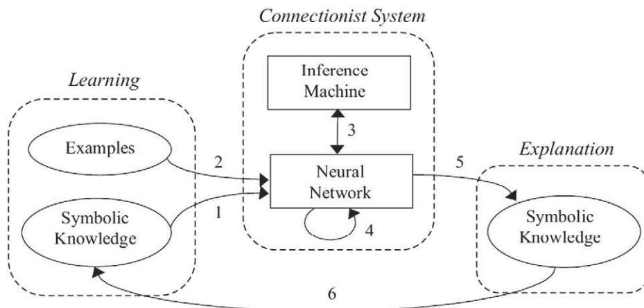
Fig. 2. Neural-symbolic learning systems [19].
