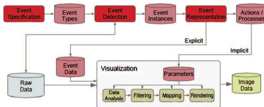
Fig. 1. The model of event-based visualization [3].
