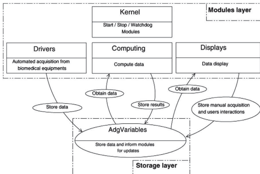
Fig. 4. Architecture of the Aiddiag 's software [4].
