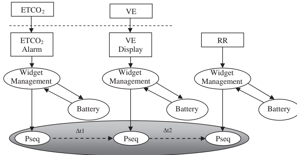
Fig. 8. A sequence of actions in a Think! network.
