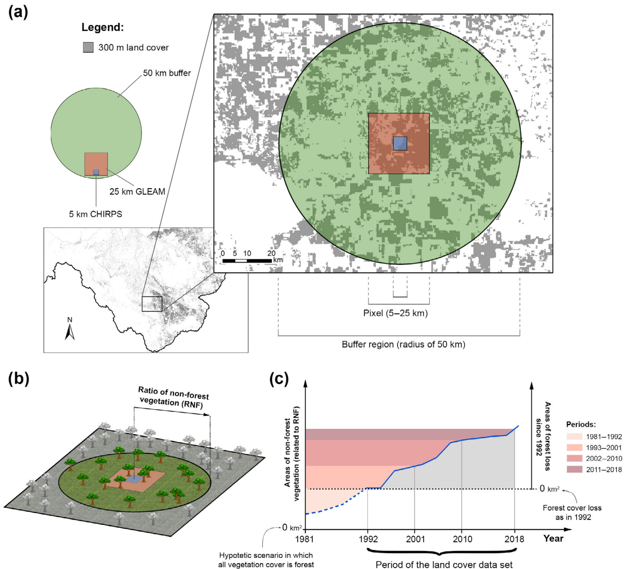
FIGURE 2 (a) Illustration of the applied methodology showing an example of the buffer zone of 50 km radio surrounding a single hydro-climatic pixel of rainfall (CHIRPS-5km) and actual-potential evapotranspiration (GLEAM-25km). The smaller pixels in grey represent the land cover change at 300 of spatial resolution. (b) Illustration of the covered area (in colours) for the ratio of non-forest vegetation (RNF). (c) Schematic representation of temporal area considerations for vegetation non-forest and forest loss since 1992. The blue line represents conceptually the value of land cover change. The periods up to which regional non-forest vegetation were set, are in red scale colours [Colour figure can be viewed at wileyonlinelibrary.com ]
