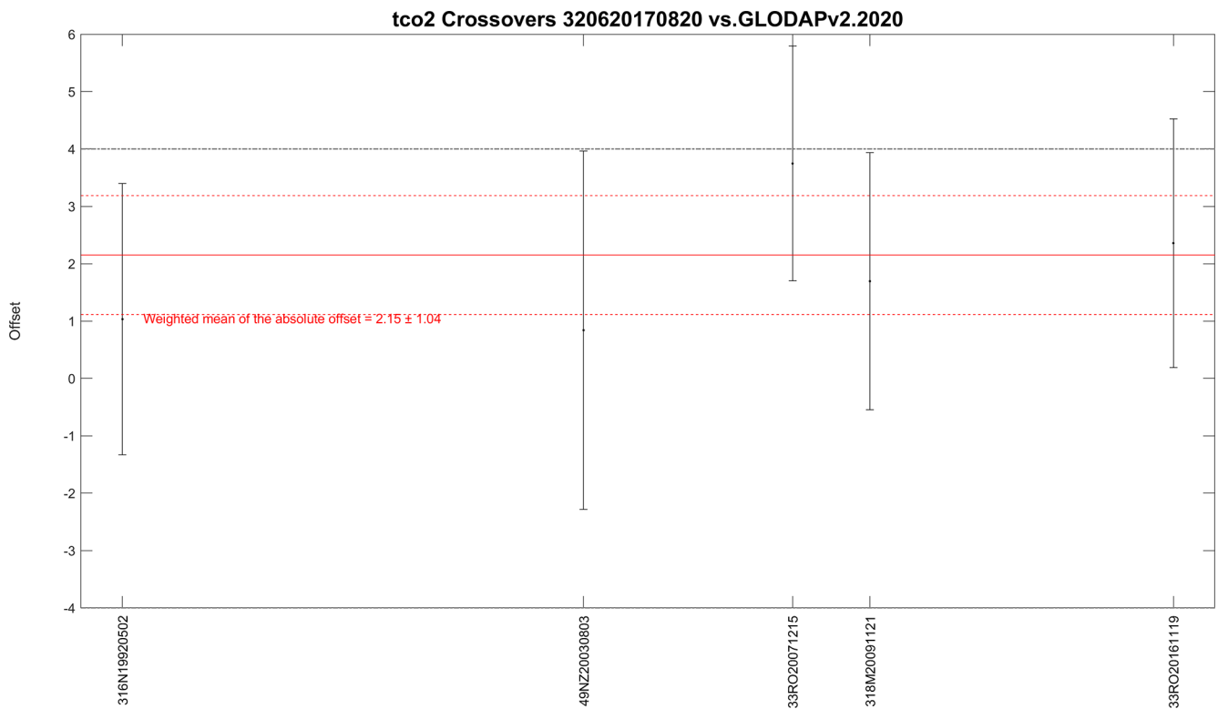
Figure 4. Example summary figure, for TCO 2 crossovers for 320620170820 versus the cruises in GLODAPv2.2020 (with cruise EX-CODE listed on the x axis sorted according to year the cruise was conducted). The black dots and vertical error bars show the weighted mean offset and standard deviation for each crossover (in \mu\text{mol kg}^{-1} ). The weighted mean and standard deviation of all these offsets are shown in the red lines and are 2.15 \pm 1.04 \mu\text{mol kg}^{-1} . The dashed black line is the reference line for a +4 \mu\text{mol kg}^{-1} offset (the corresponding line for -4 \mu\text{mol kg}^{-1} offset is right on top of the x axis and not visible).
